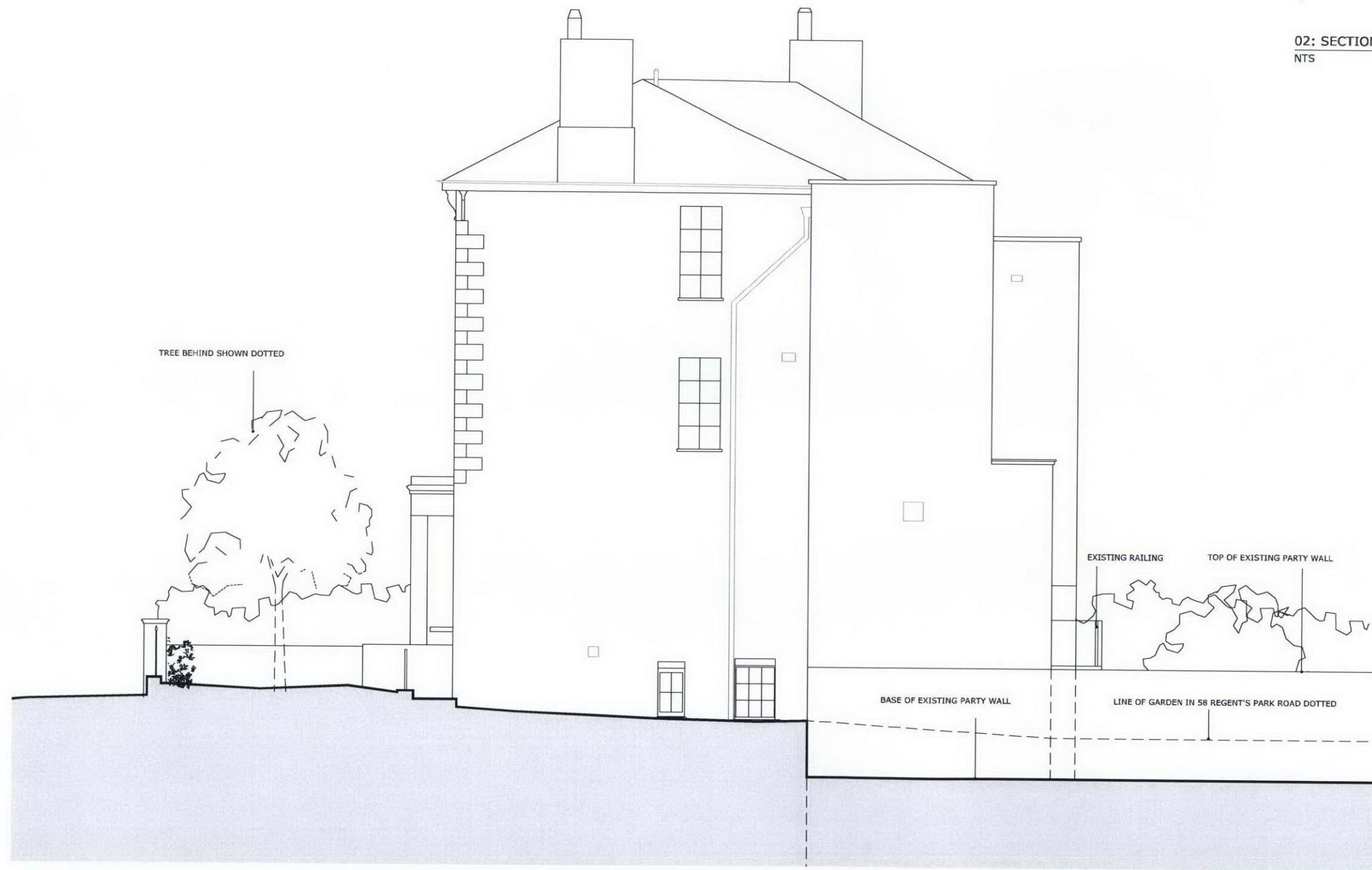
01: EAST ELEVATION SCALE 1:50 at A1
