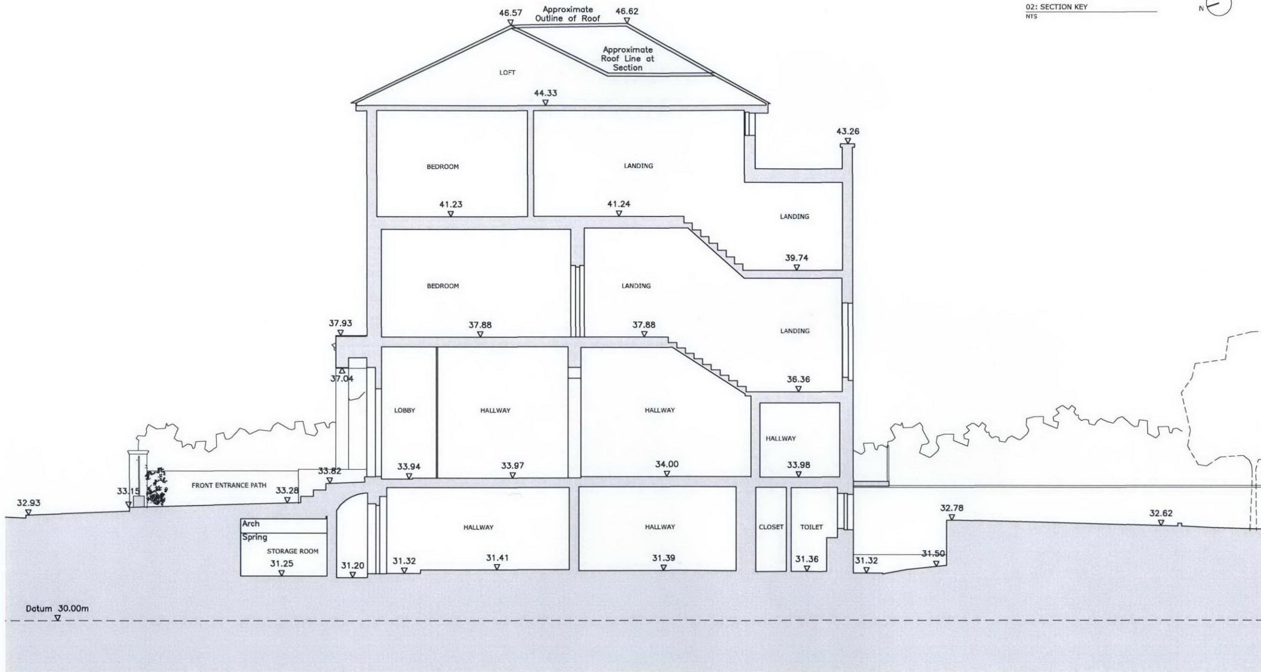
01: CROSS SECTION Y-Y SCALE 1:50 at A1
