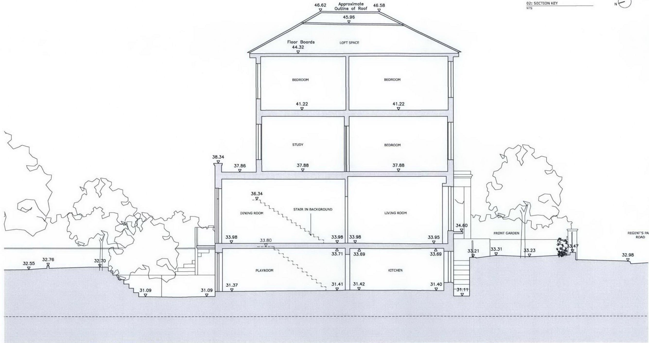
01: CROSS SECTION X-X SCALE 1:50 at A1
