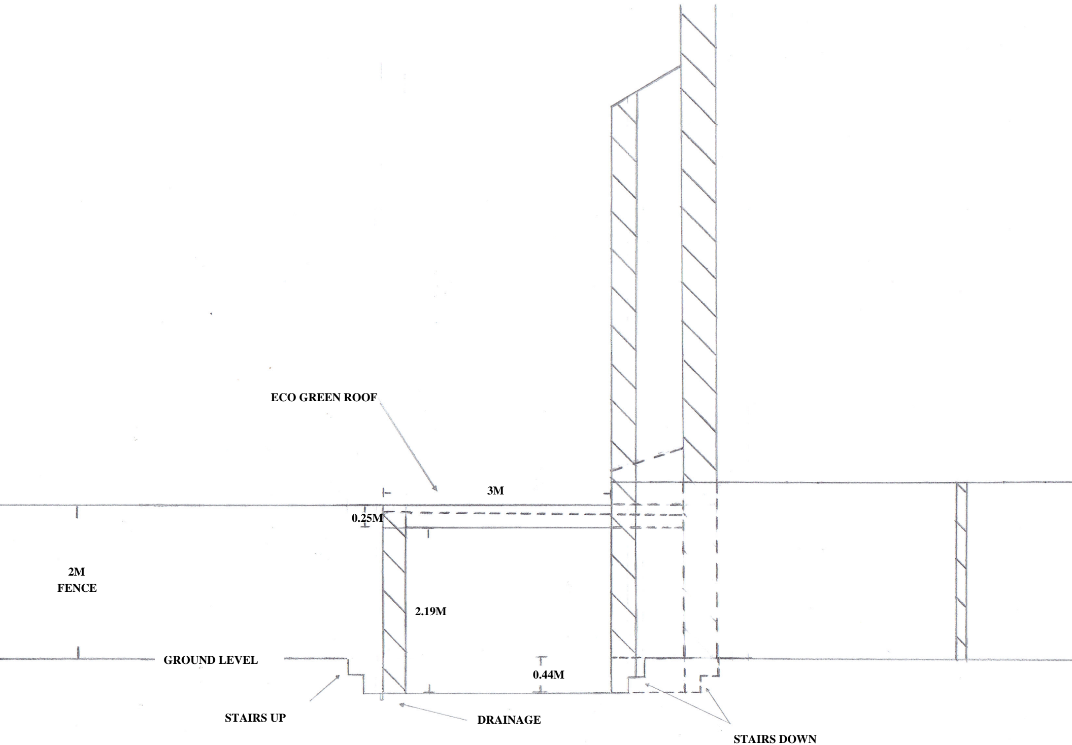
PROPOSED GARDEN FLAT SIDE CUT SCALE 1:50
