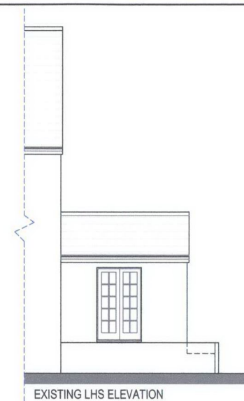
EXISTING LHS ELEVATION
