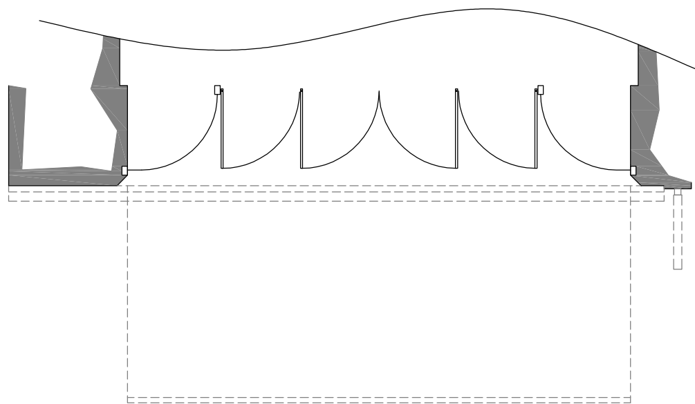
GROUND FLOOR PLAN (part)
