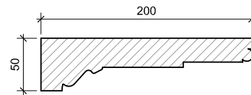
ARCHITRAVE TYPE - A2
