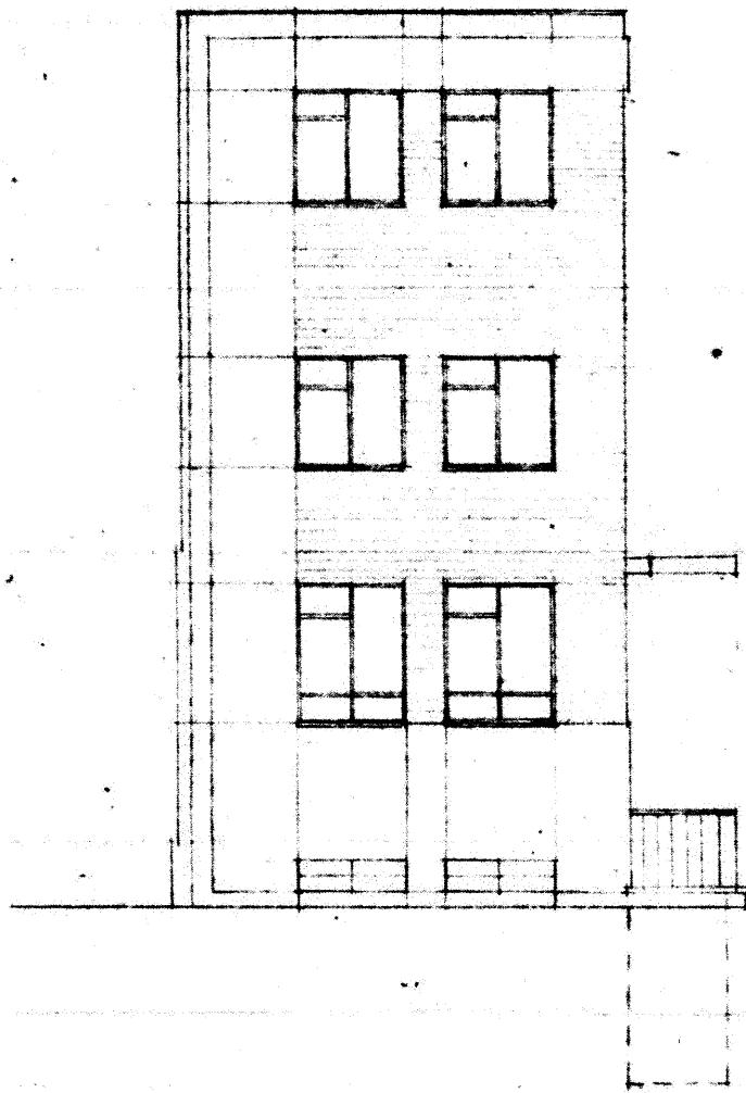
COLVILLE PLACE ELEVATION
