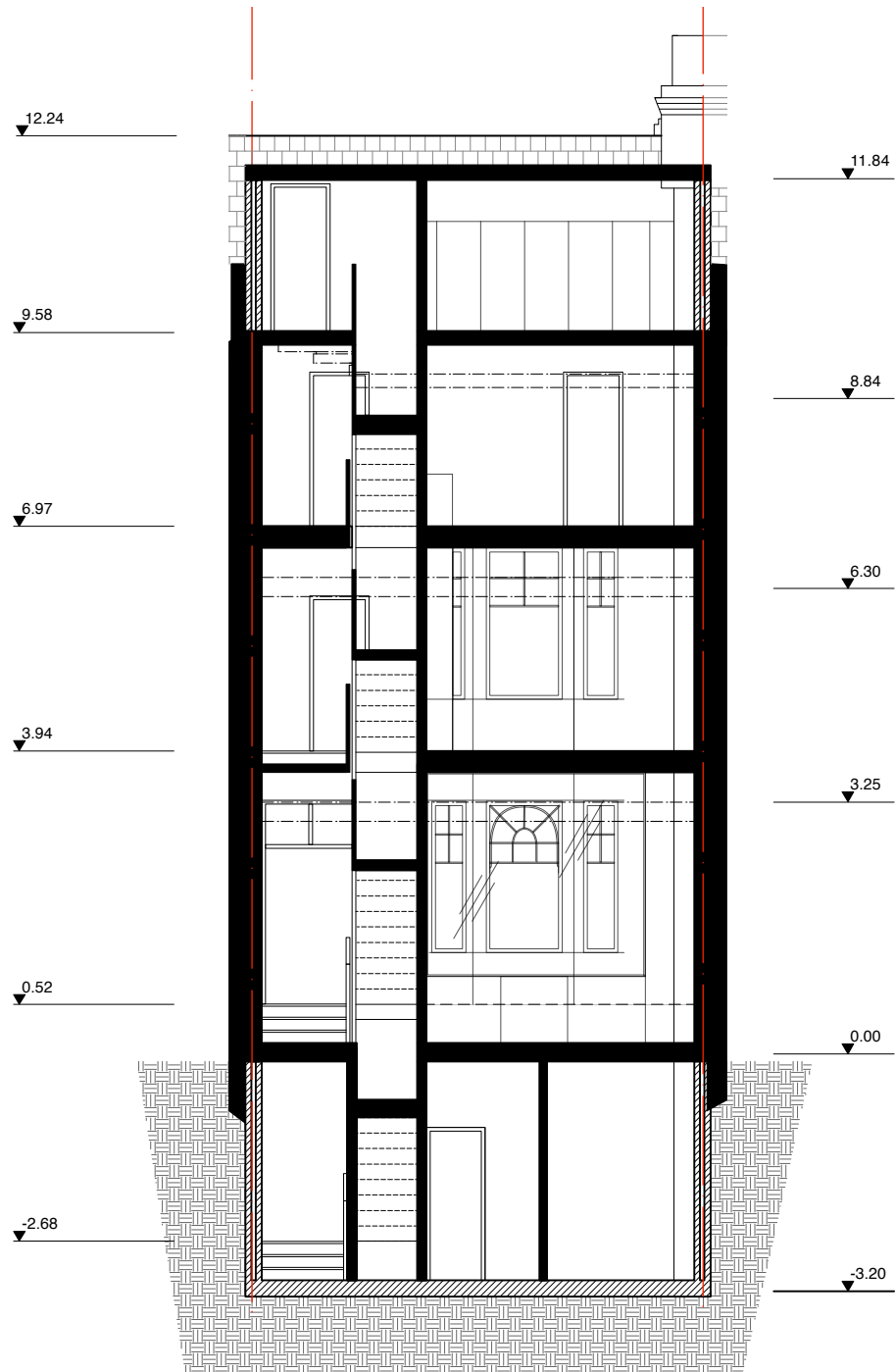
CROSS SECTION - PROPOSED
