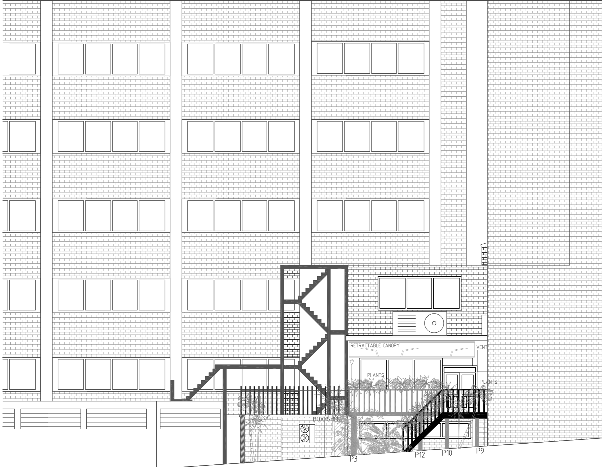
UPDATED EXISTING REAR ELEVATION
