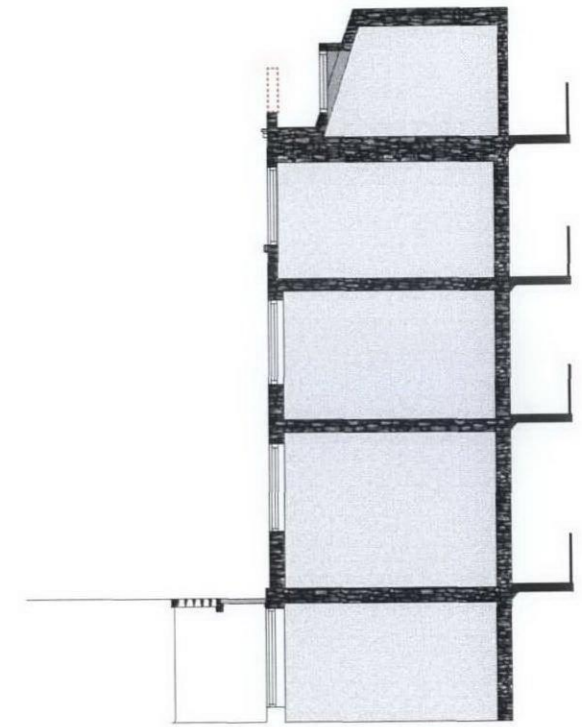
Approved Section A-A'
