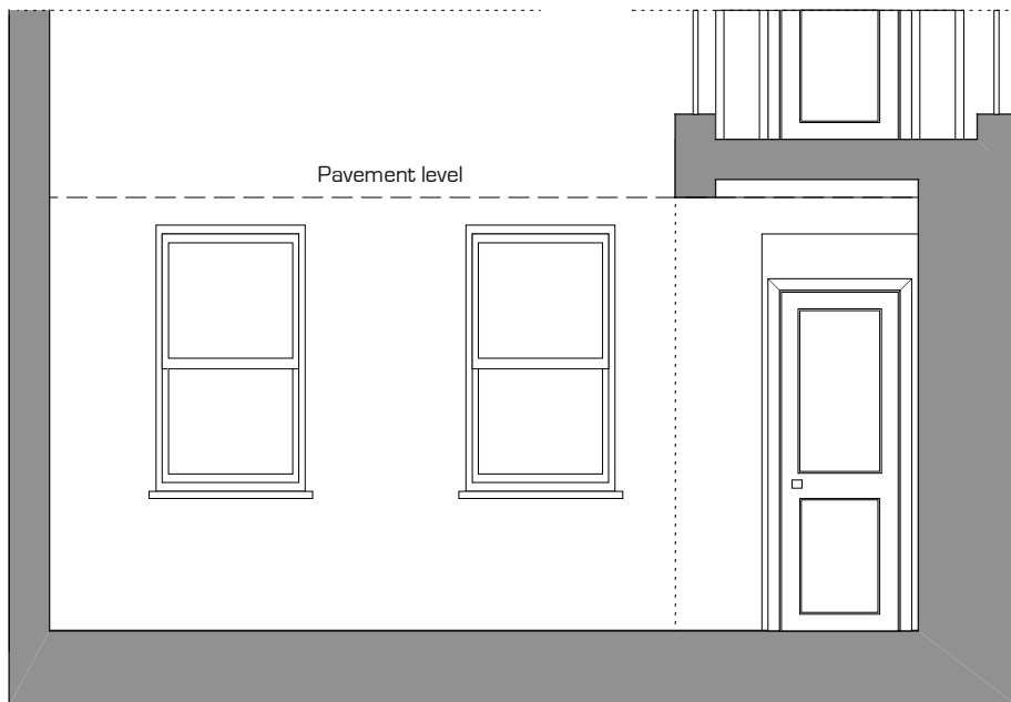
Existing Front Elevation FF
