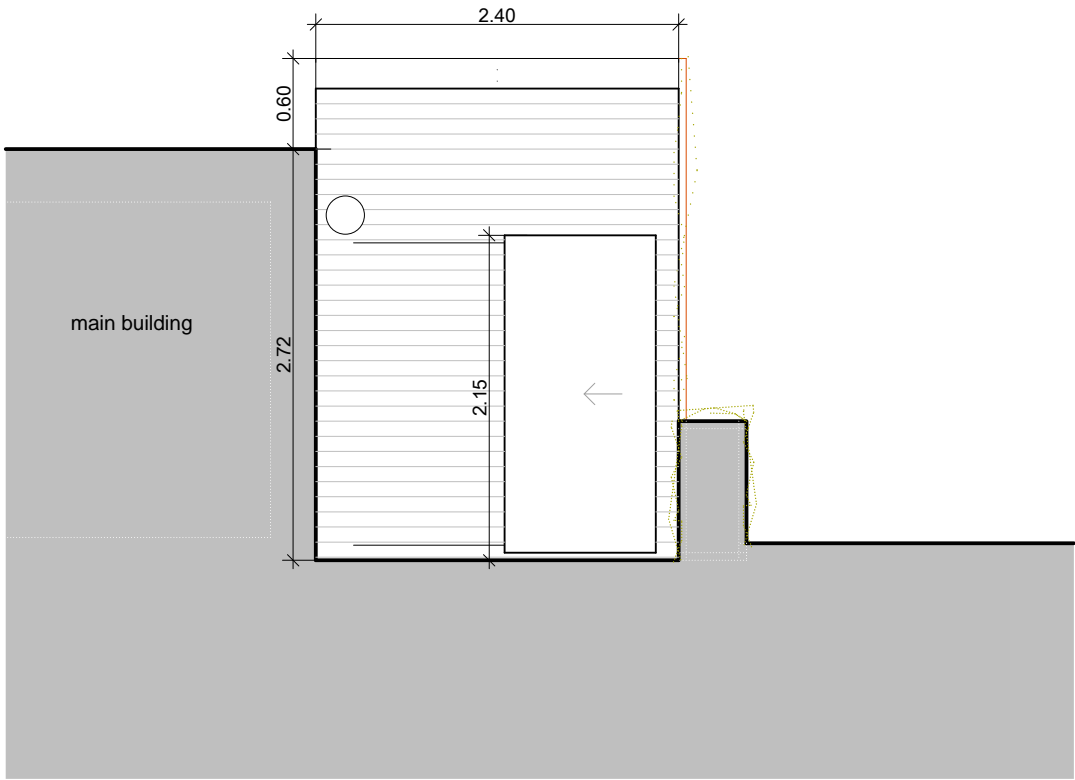
cross elevation looking west
