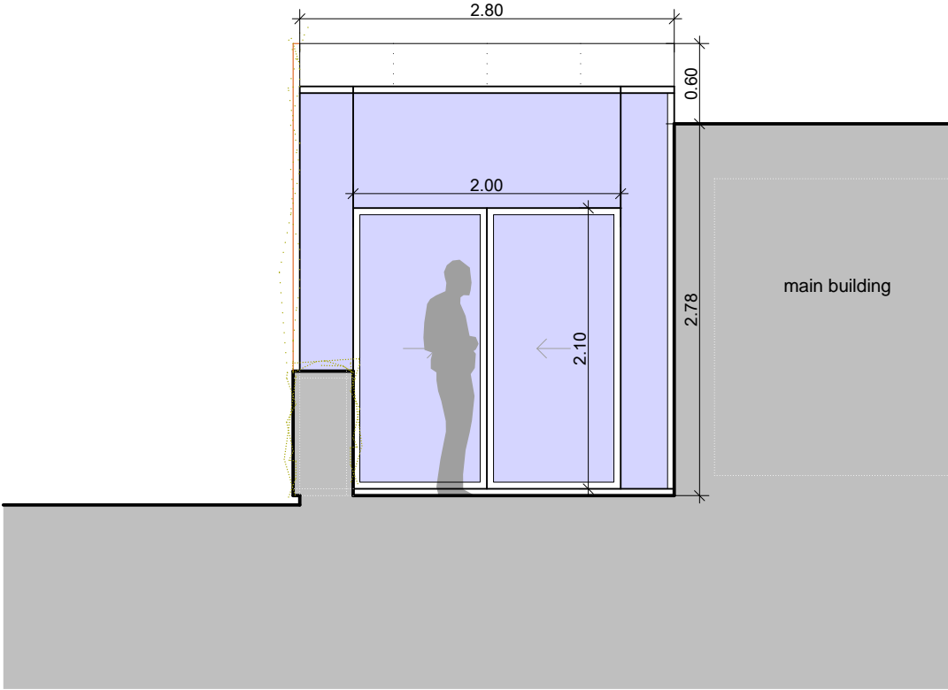
cross elevation looking east
