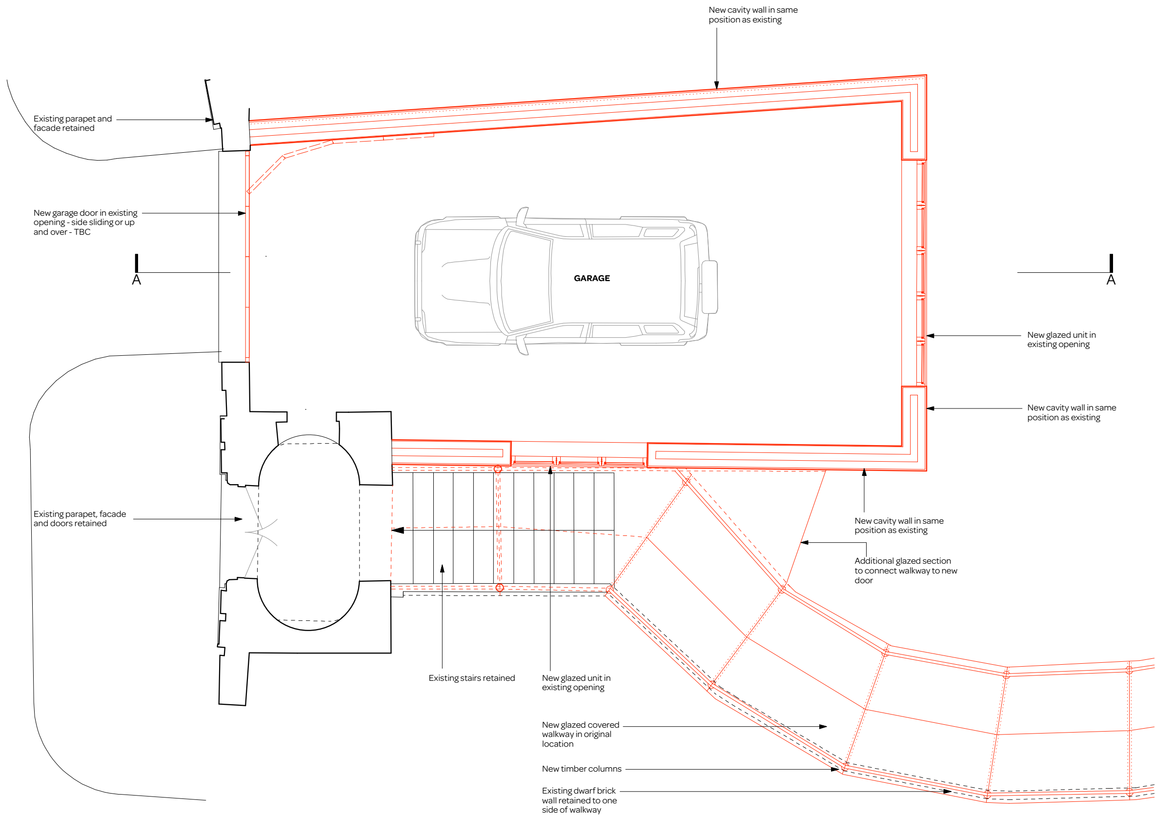
PROPOSED UPPER GROUND FLOOR PLAN
