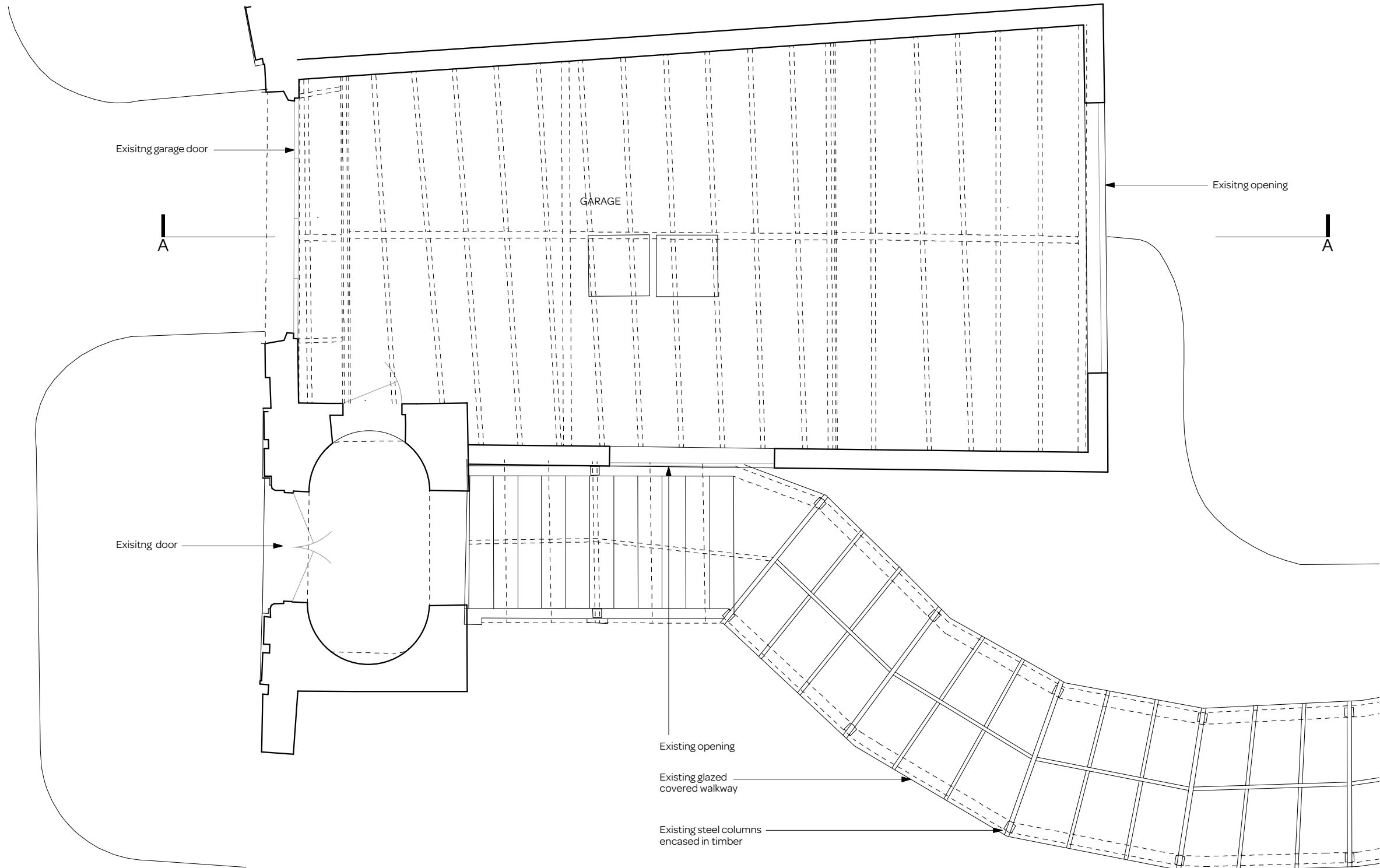
EXISTING UPPER GROUND FLOOR PLAN
