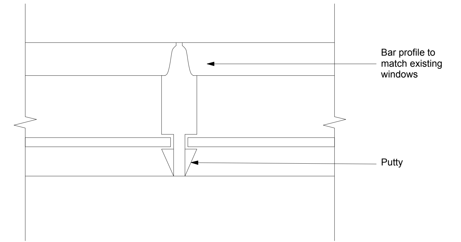
GLAZING BAR SECTION (PLAN)
