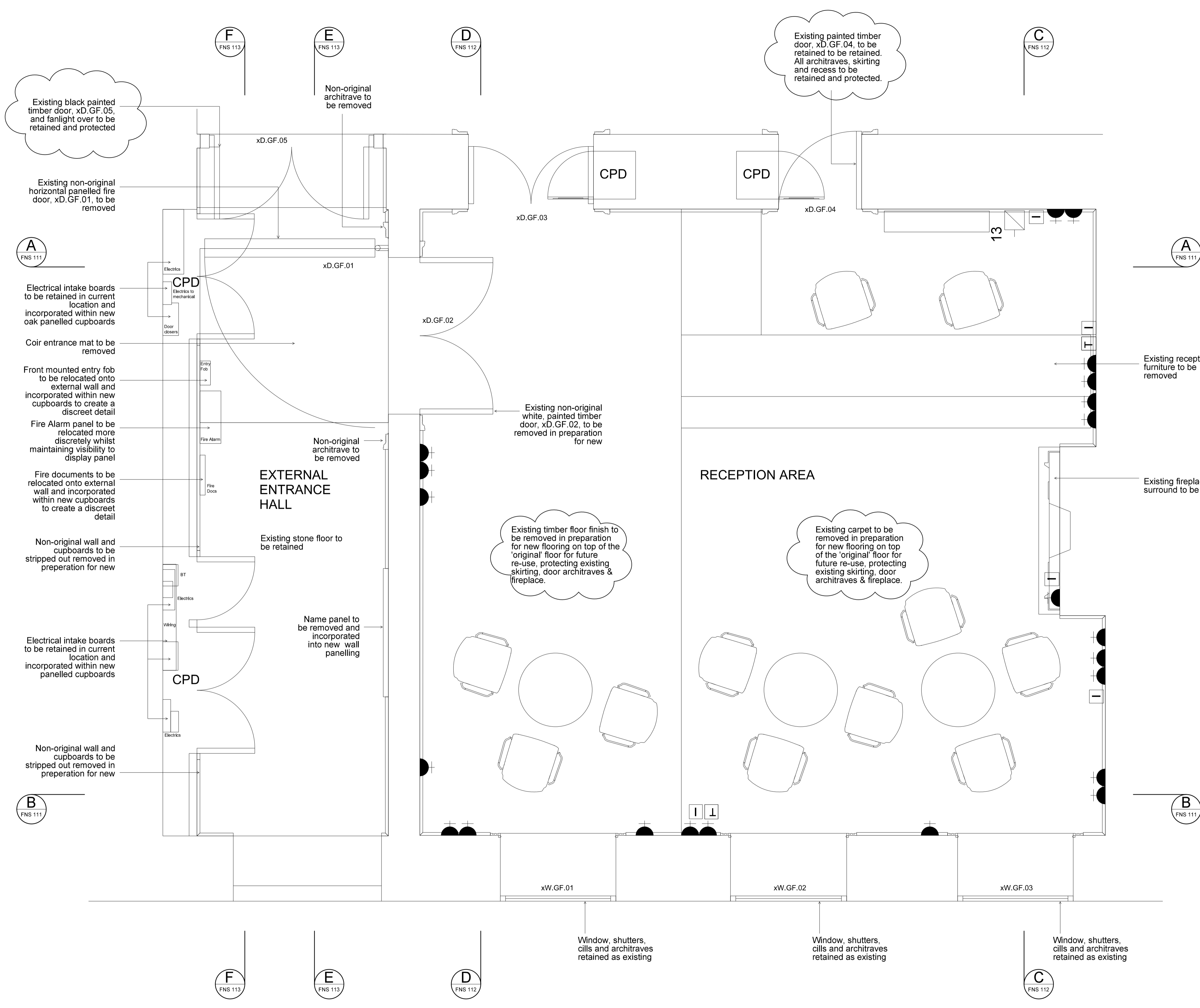
EXISTING GROUND FLOOR PLAN
