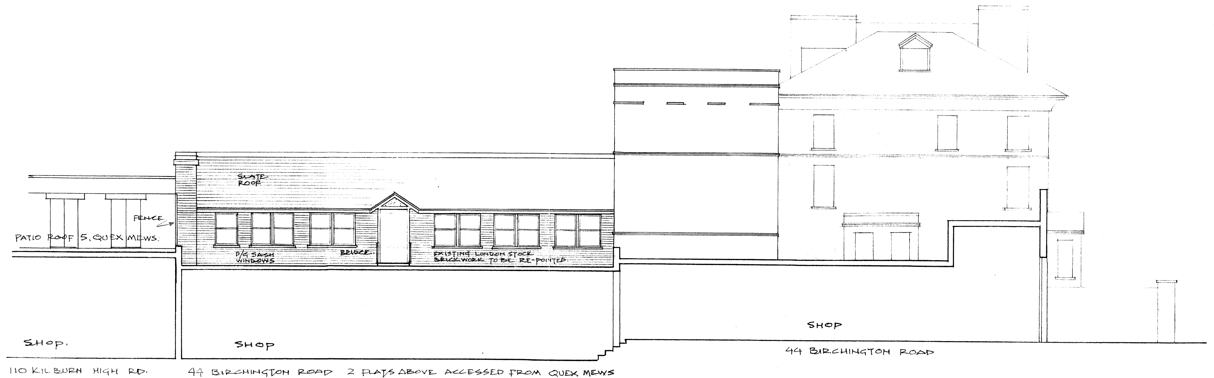
PROPOSED ELEVATION SOUTH.
