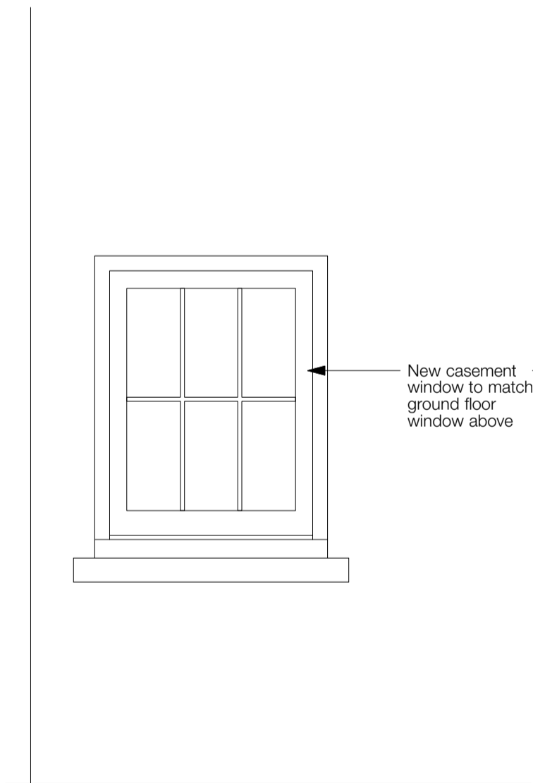
PROPOSED ELEVATION
