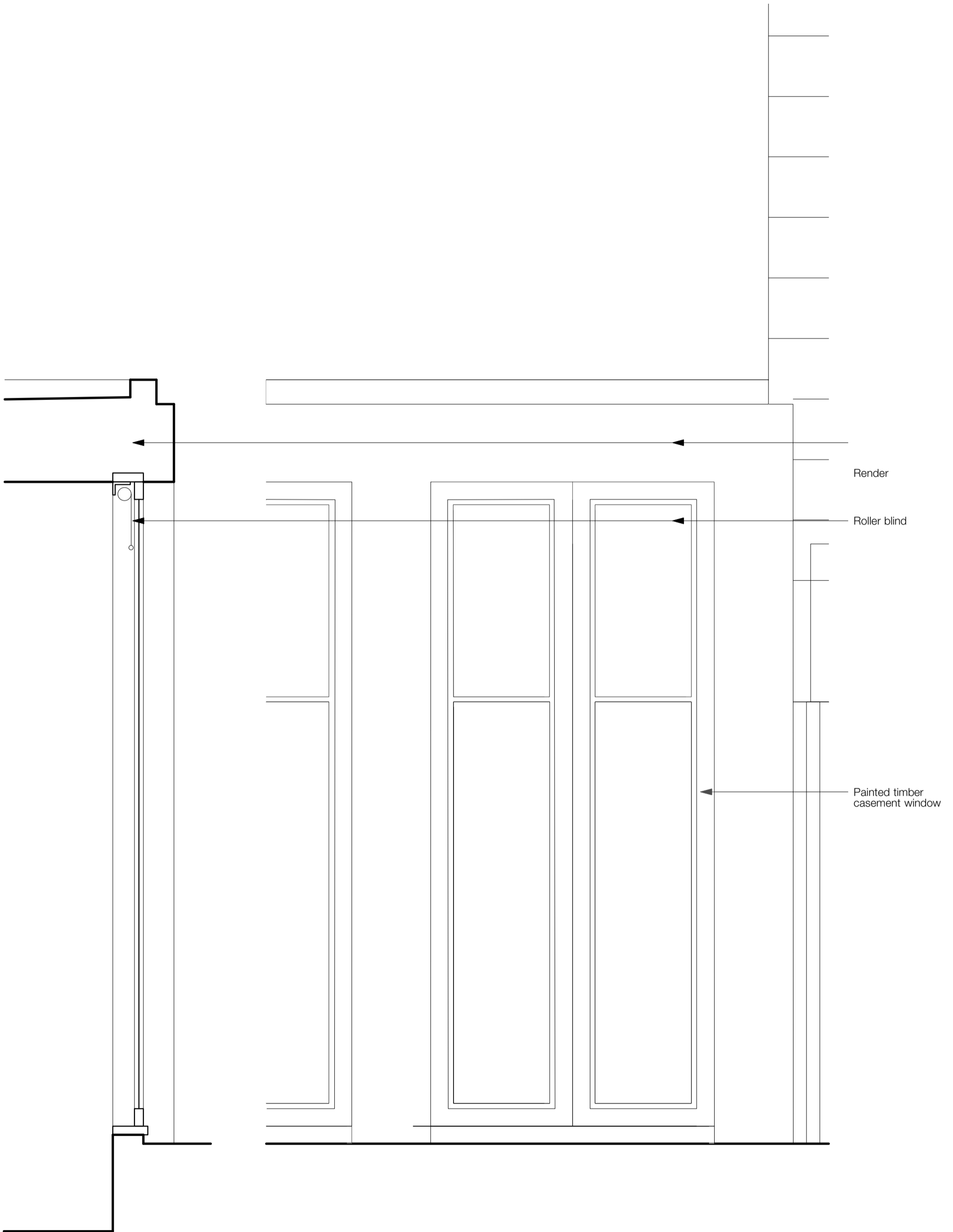
SECTION OF WEST WALL
