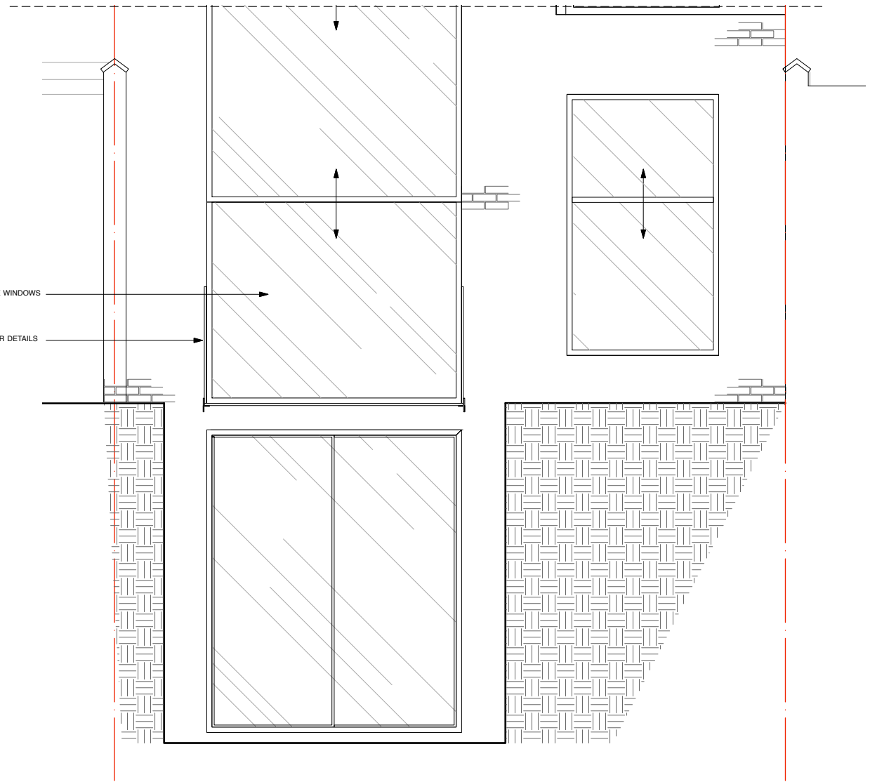
PROPOSED REAR ELEVATION - showing bridge
