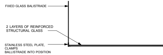
PROPOSED SECTION AA
