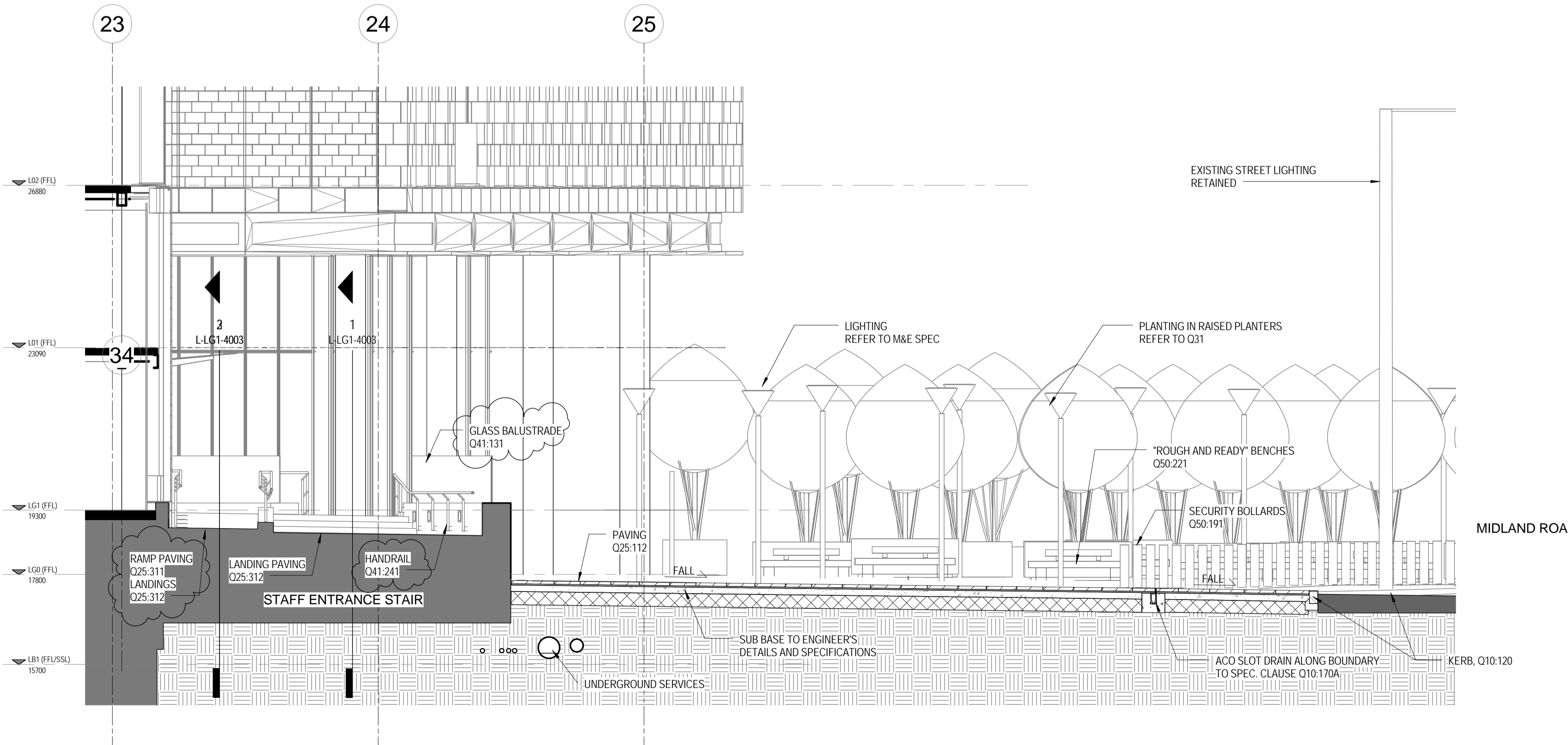
② LONG CROSS SECTION THROUGH MAIN STAIR TO KERB 1 : 75
