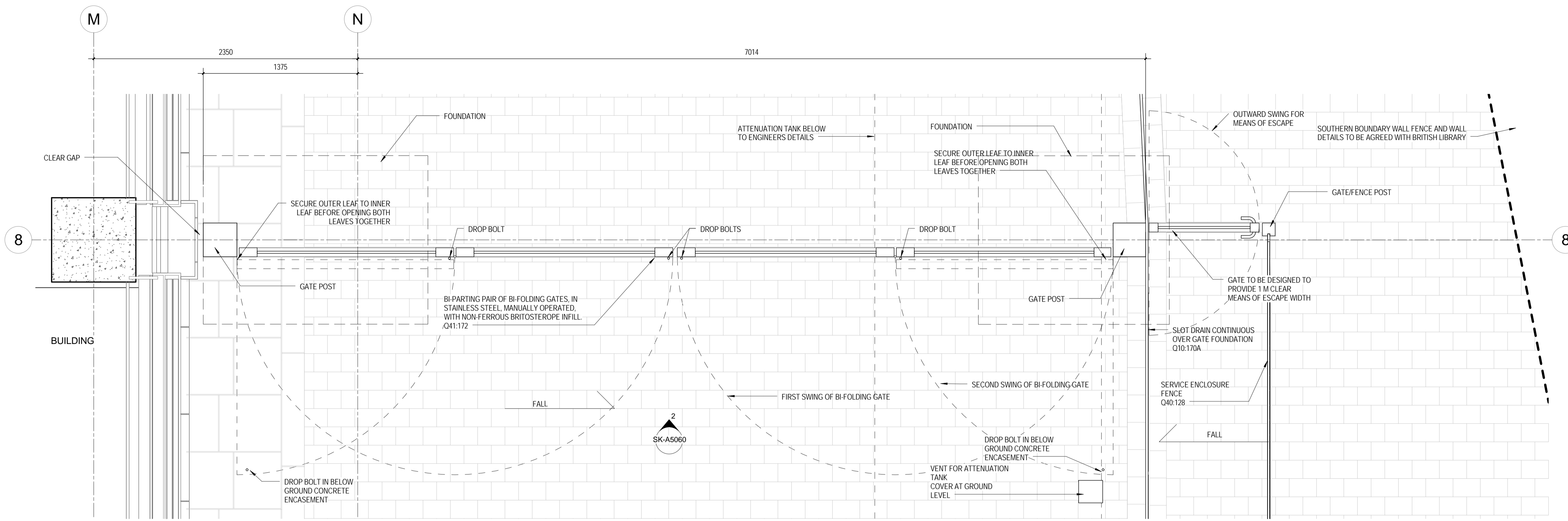
1 PERMEABILITY ROUTE- NON-FERROUS GATE 2 PLAN 1:20
