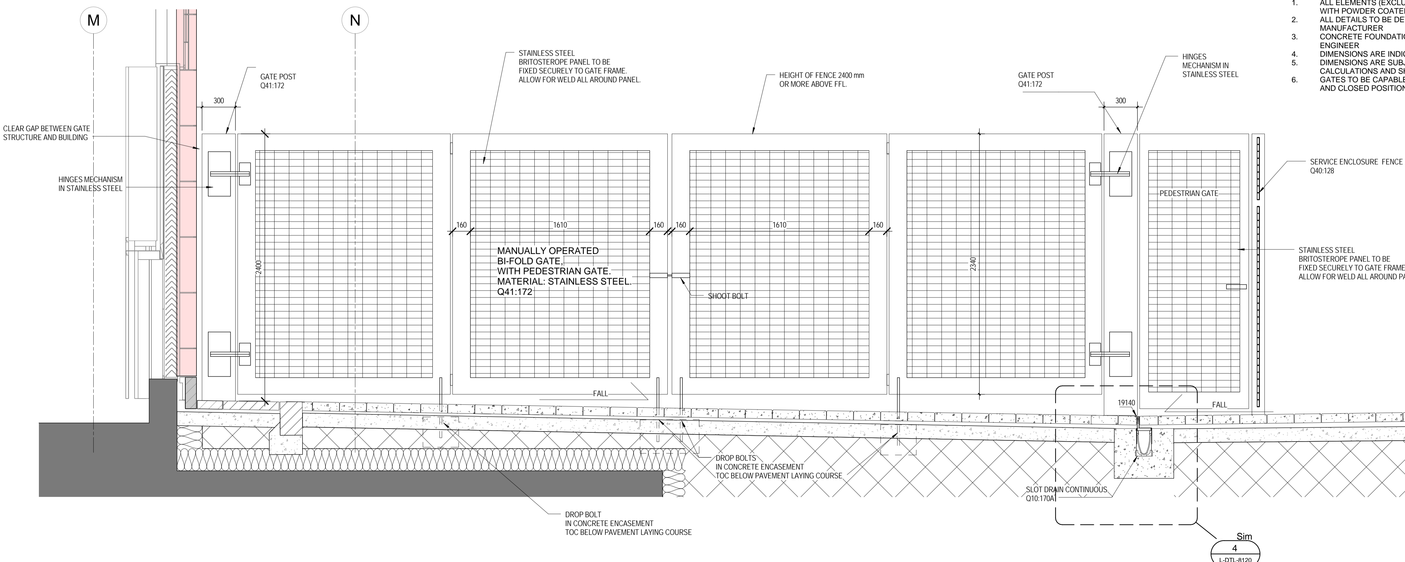
2 PERMEABILITY ROUTE - NON FERROUS GATE2 ELEVATION 1:20
