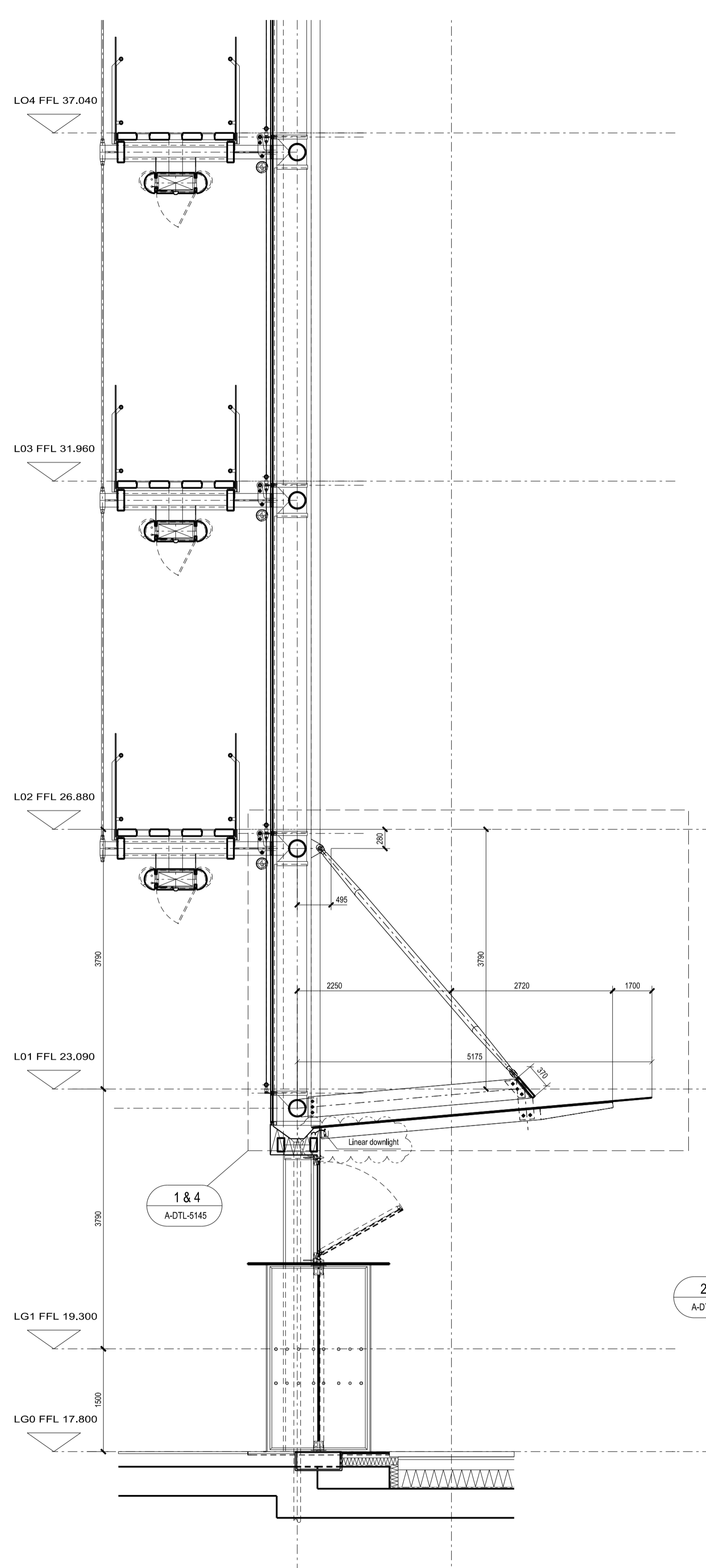
2 Section 1:50
