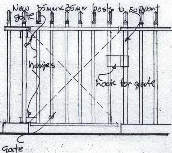
Gate detail
