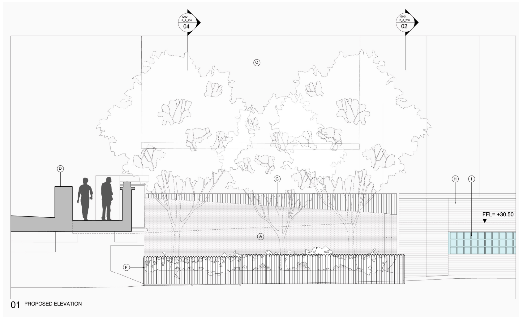
Fig. 15 Proposed elevation (please see AHMM drawing 12001_P_A_231)
