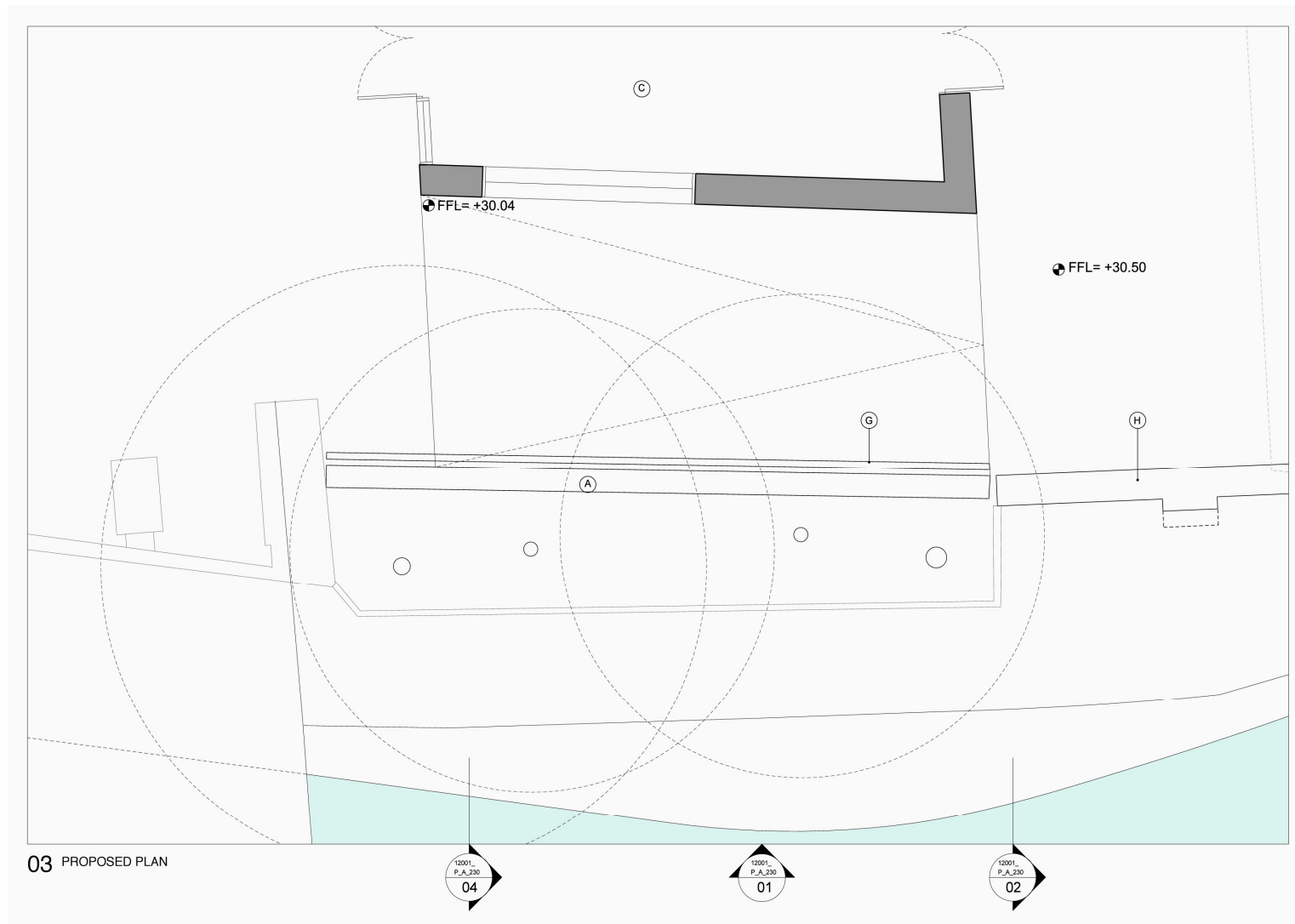
Fig. 14 Proposed plan (please see AHMM drawing 12001_P_A_231)
