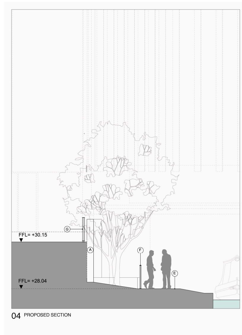
Fig. 16 Proposed cross section (please see AHMM drawing 12001_P_A_231)
