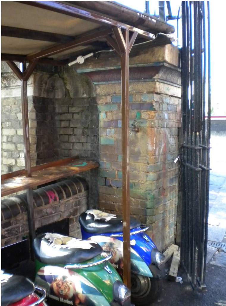
Fig. 5 The existing wall abuts up against the Hampstead Road Bridge
