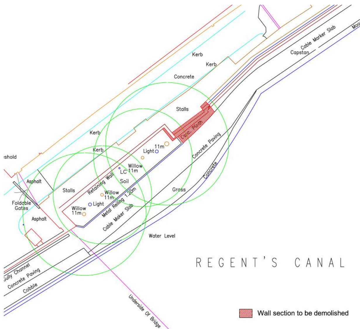
Fig. 13 Detail in plan of the existing parapet joining the end of the abutment.
