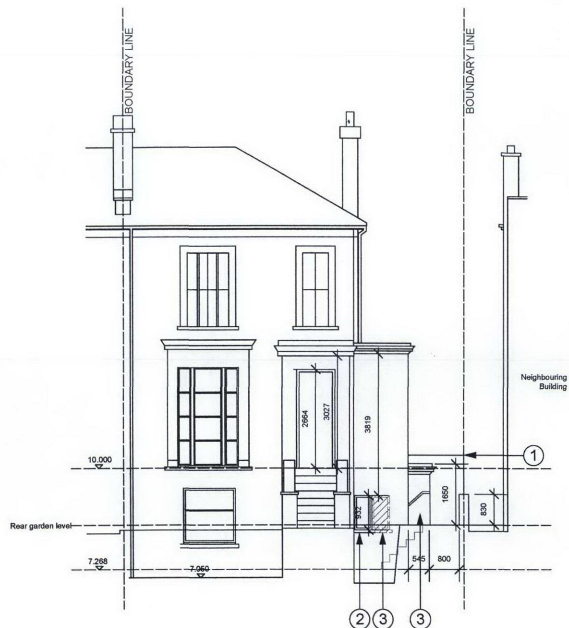
FRONT ELEVATION
