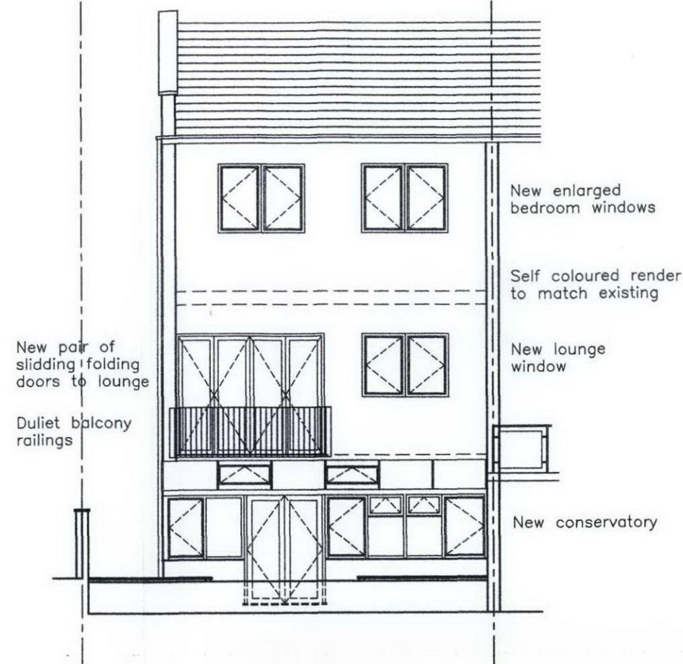
Rear Elevation
