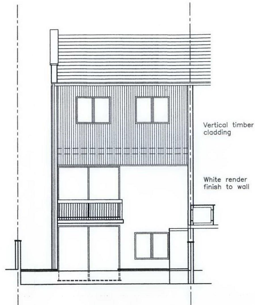
Rear Elevation
