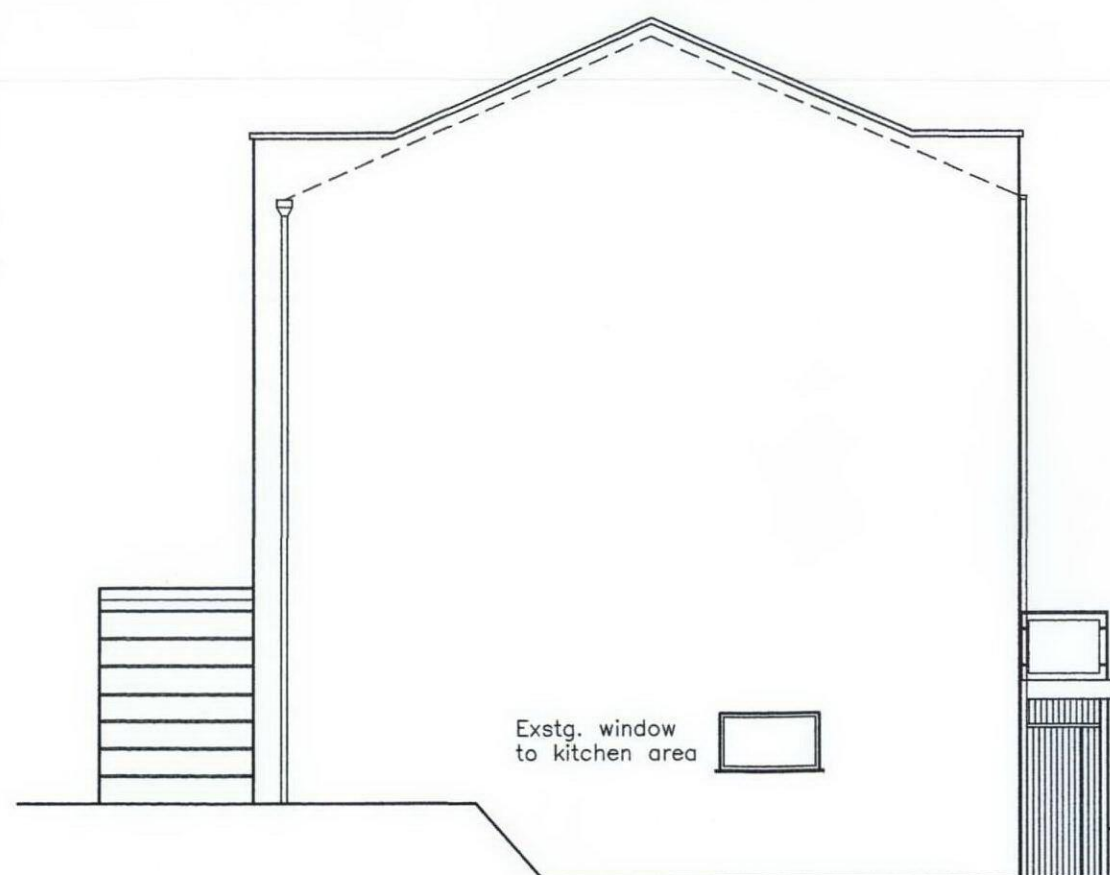
Side Elevation
