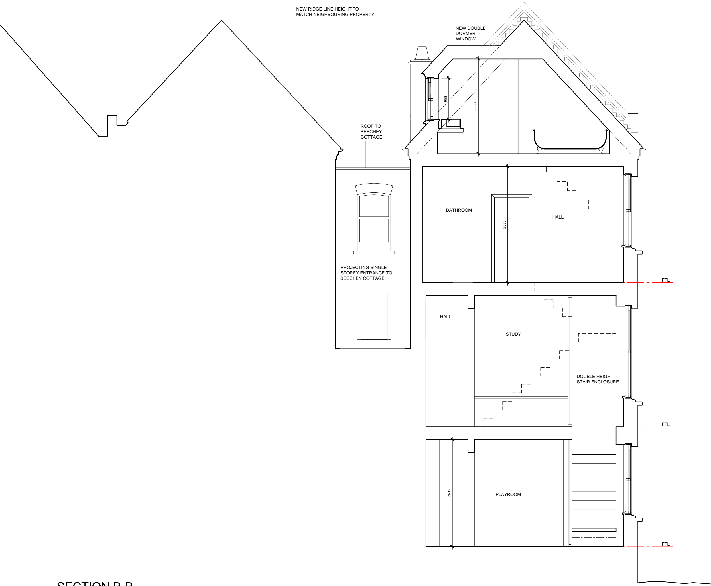
SECTION B-B
