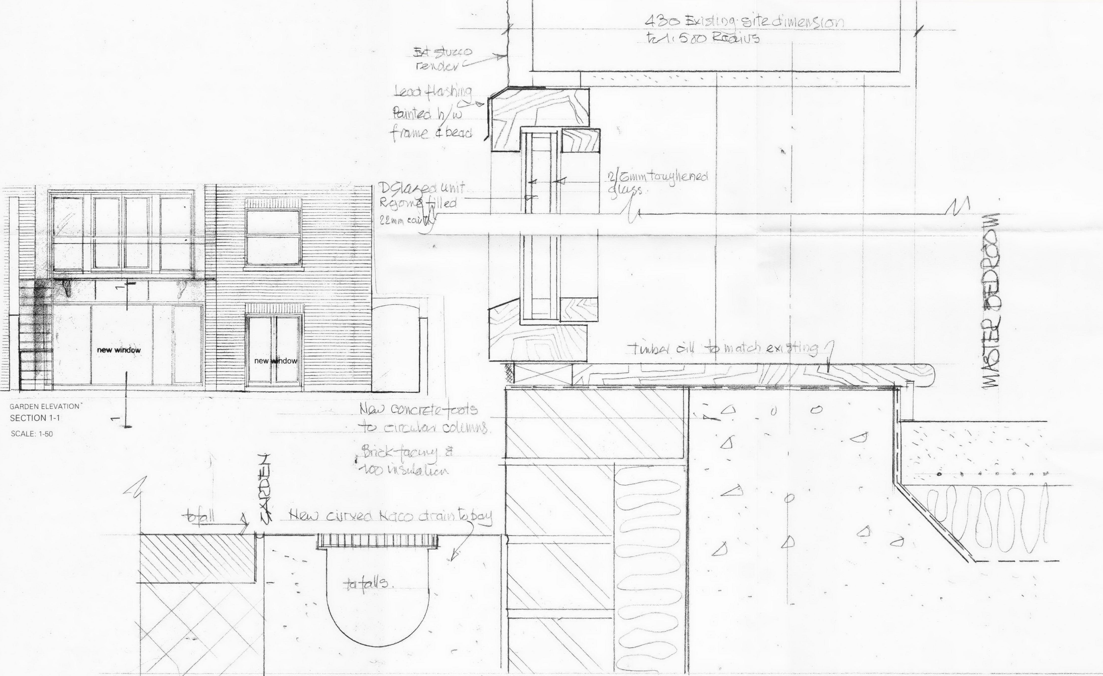
SECTION 1-1 above. 1-1. SECTION THRO' CURVED BAY WINDOW 1/2 Full Size @ A2 14 BELSIZE PARK GARDENS
