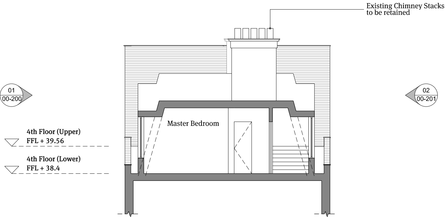
01 Proposed Section AA 1:100 @ A3
