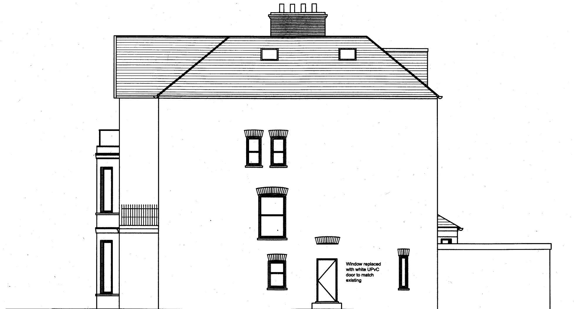
PROPOSED SIDE ELEVATION ADJACENT TO 49 HELENA COURT
