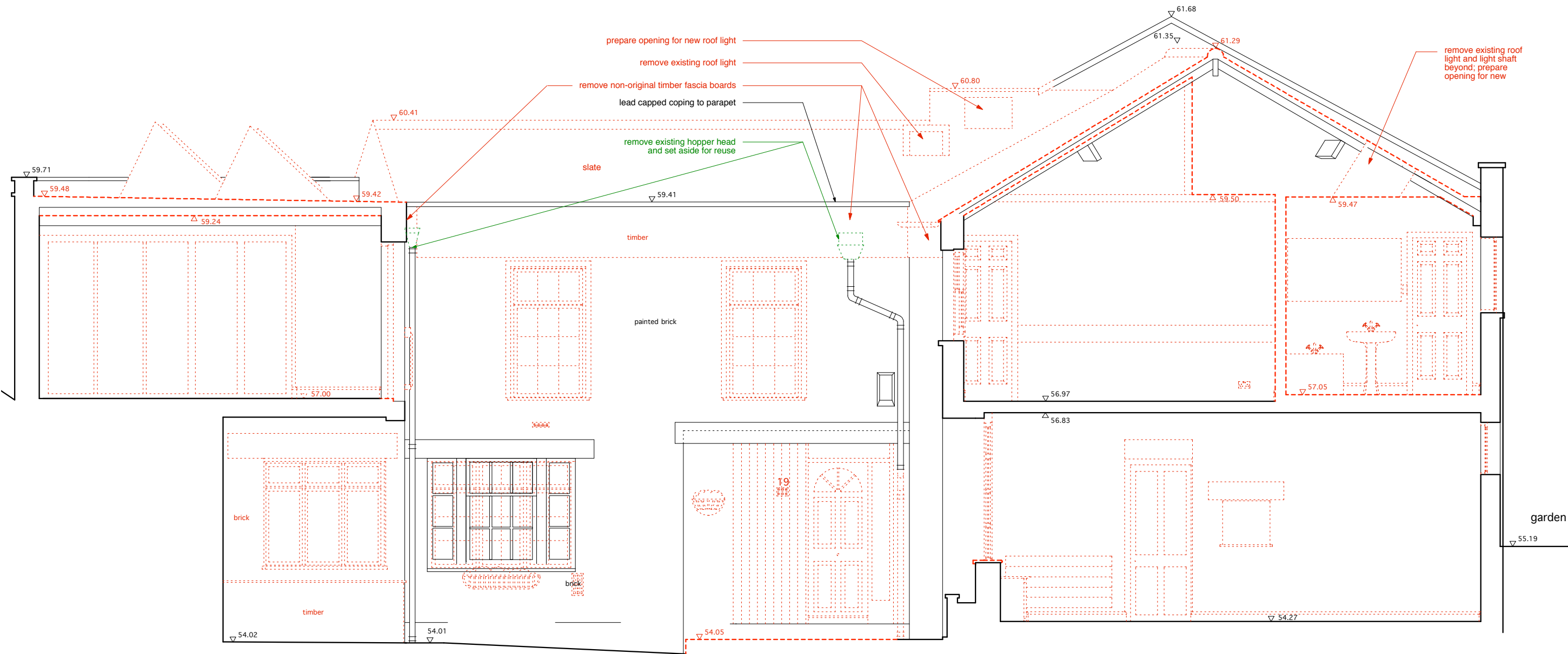
SECTION B-B △ 53.00m A.O.D.
