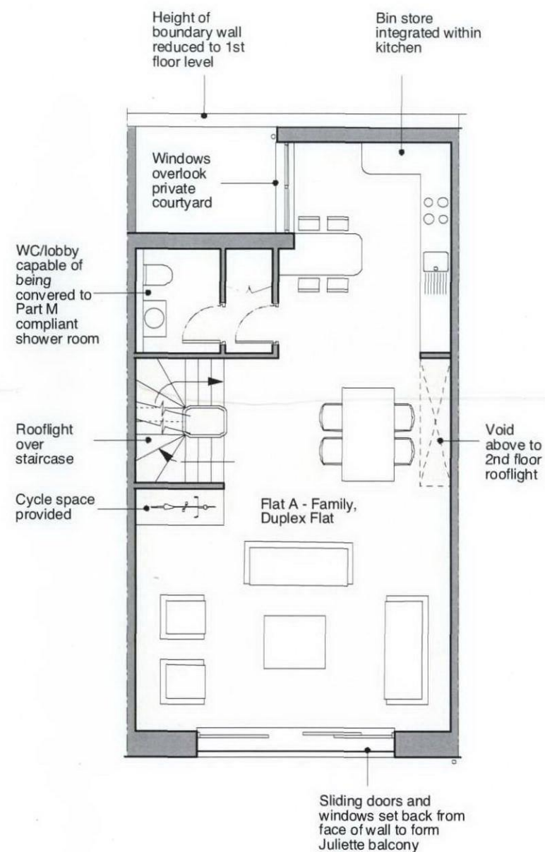
1ST FLOOR, FLAT A
