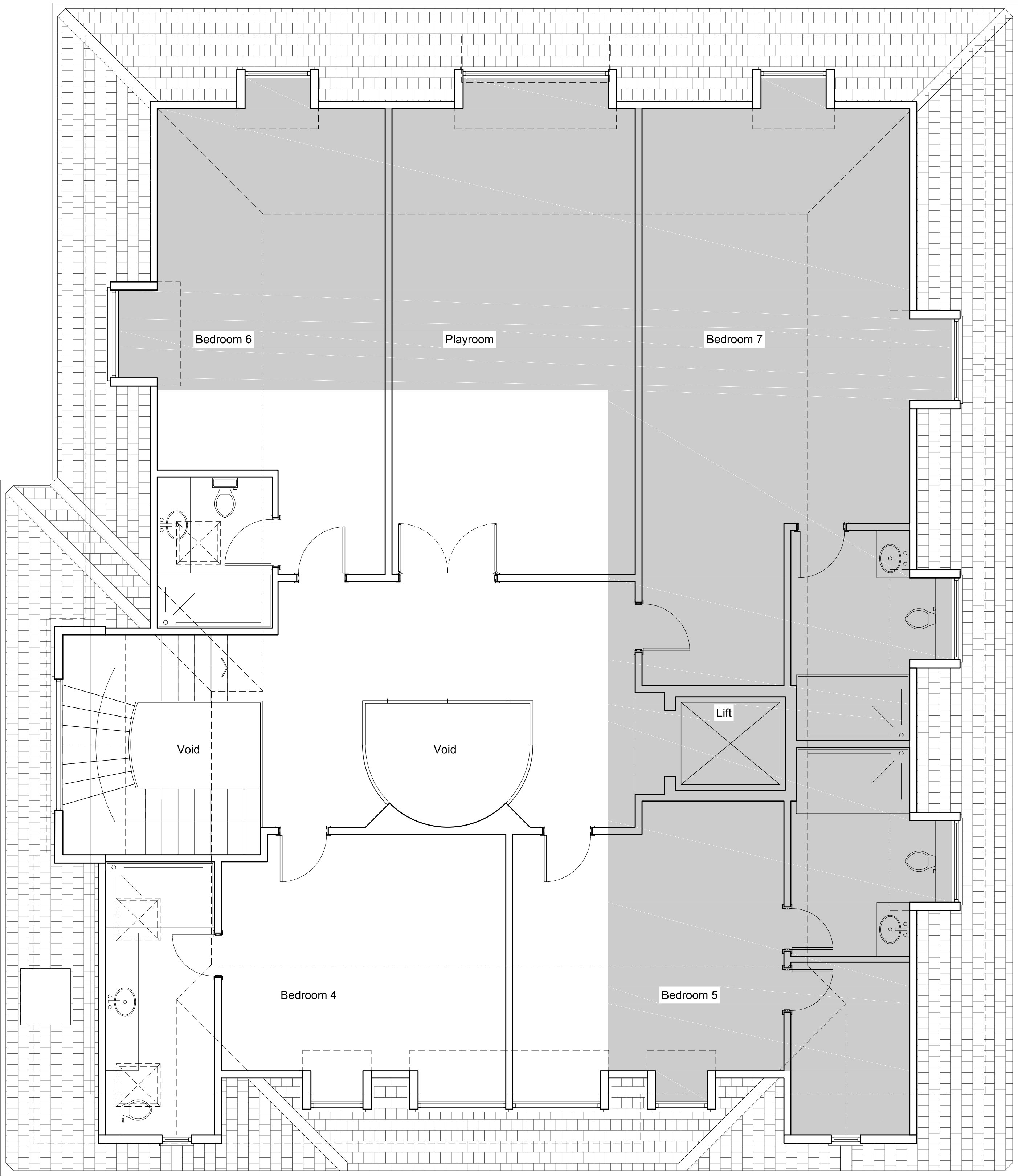
Proposed Second Floor Scale 1:50
