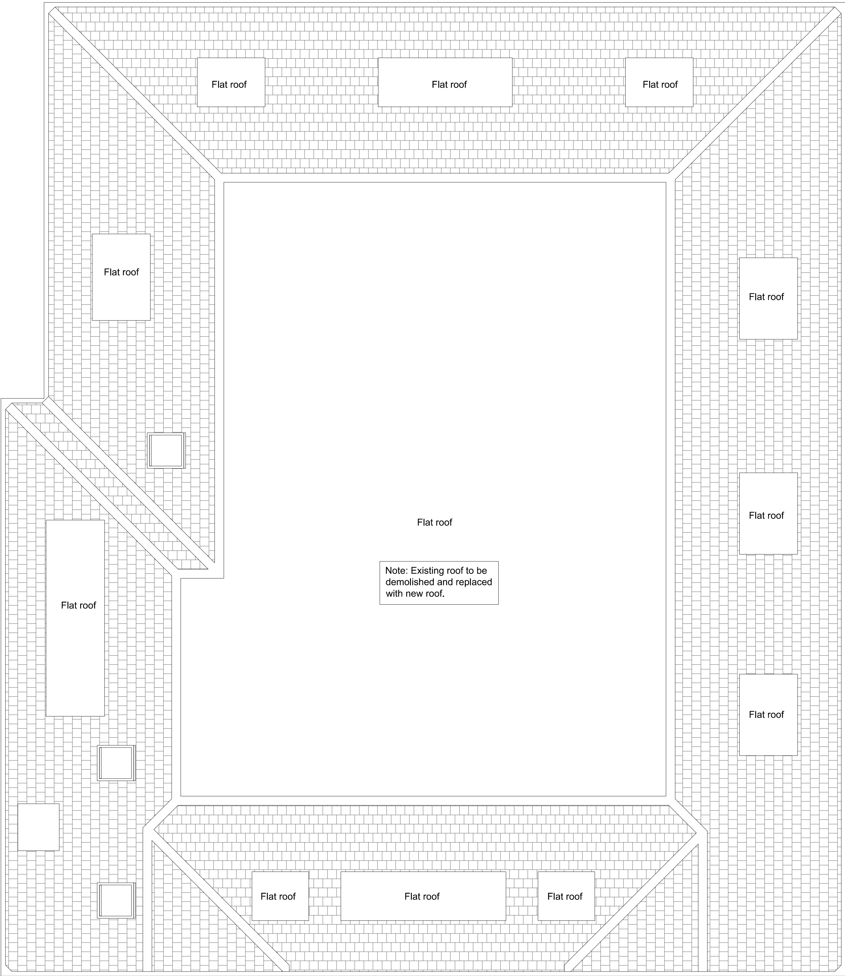
Proposed Roof Scale 1:50
