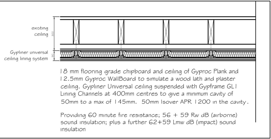
Typical floor section showing ceiling lining between flats @ 1/20 scale
