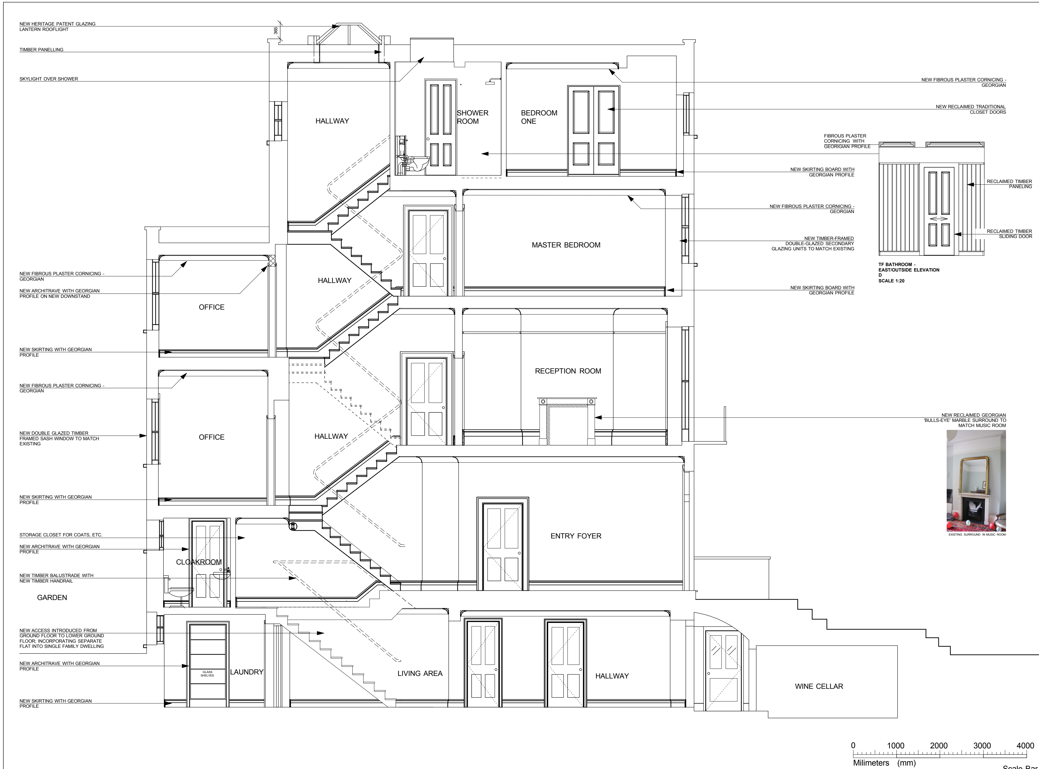
SECTION AA PROPOSED
