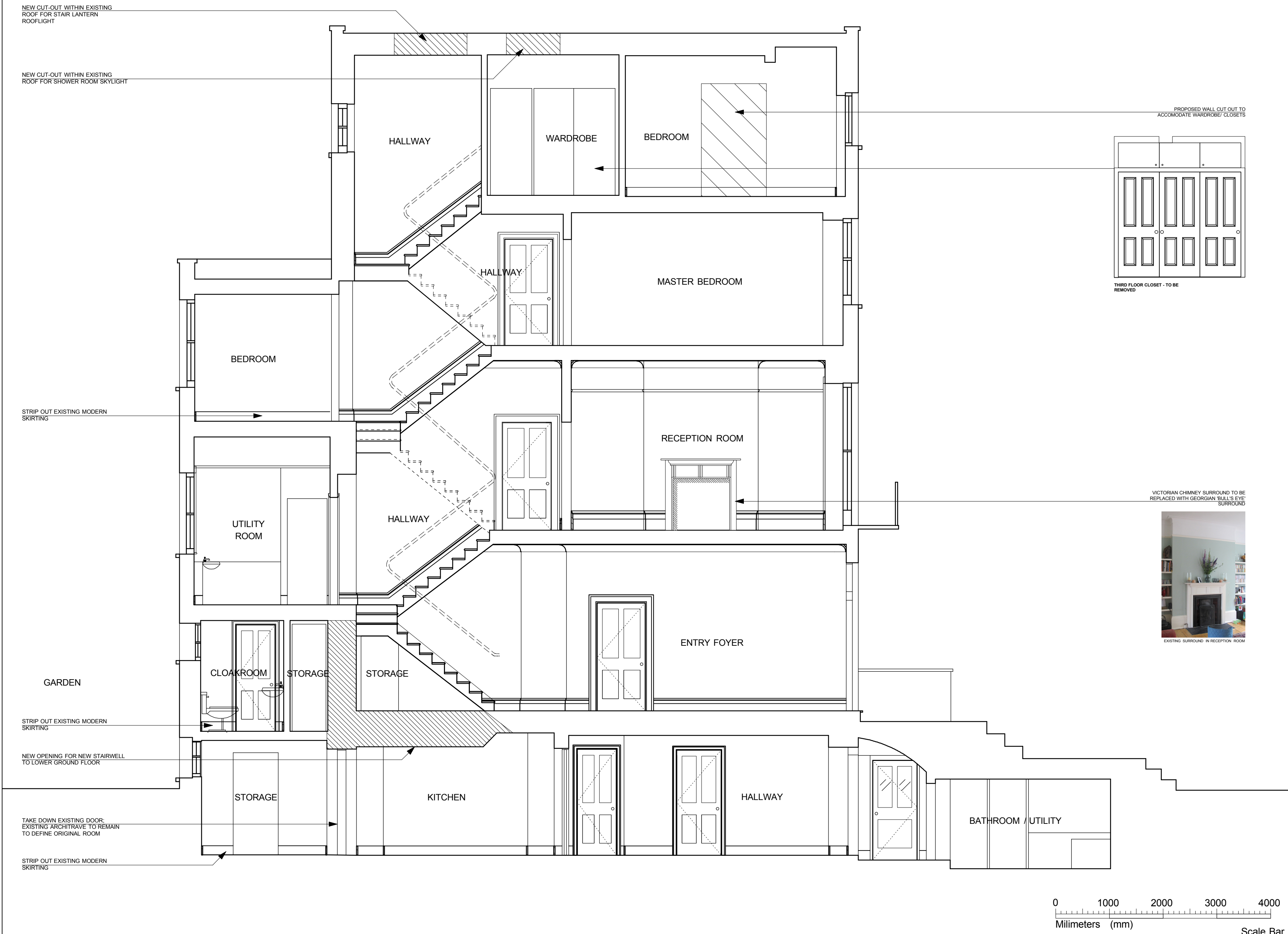
SECTION AA EXISTING
