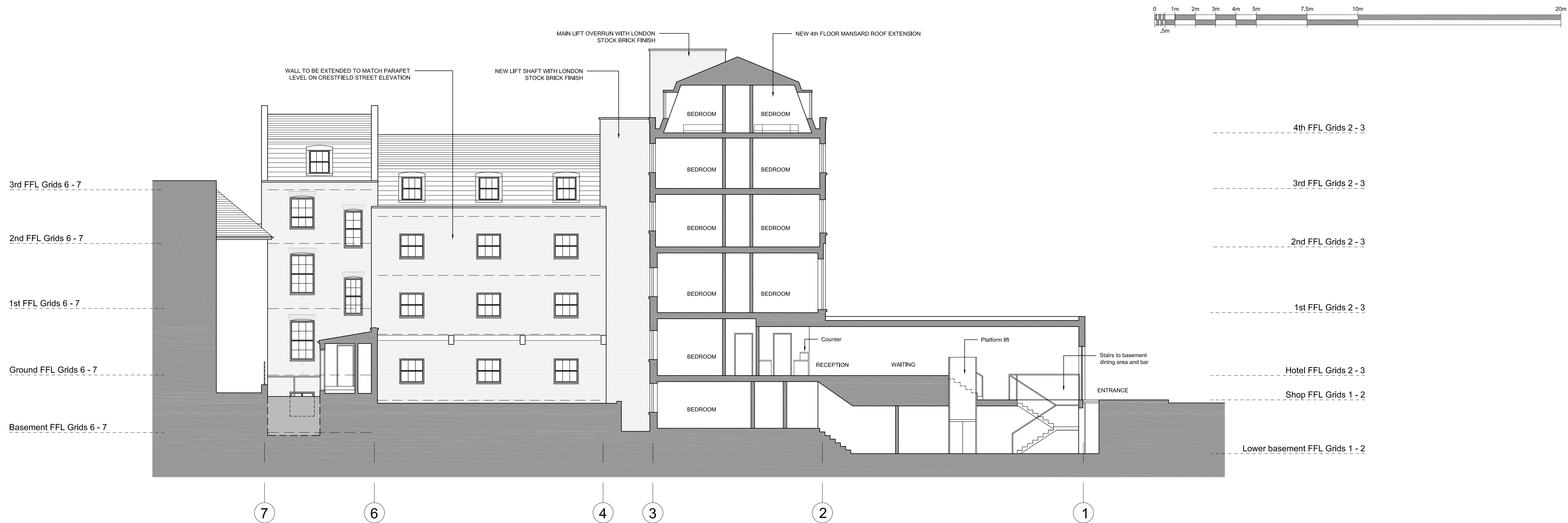
SECTION B - B, REAR OF CRESTFIELD STREET
