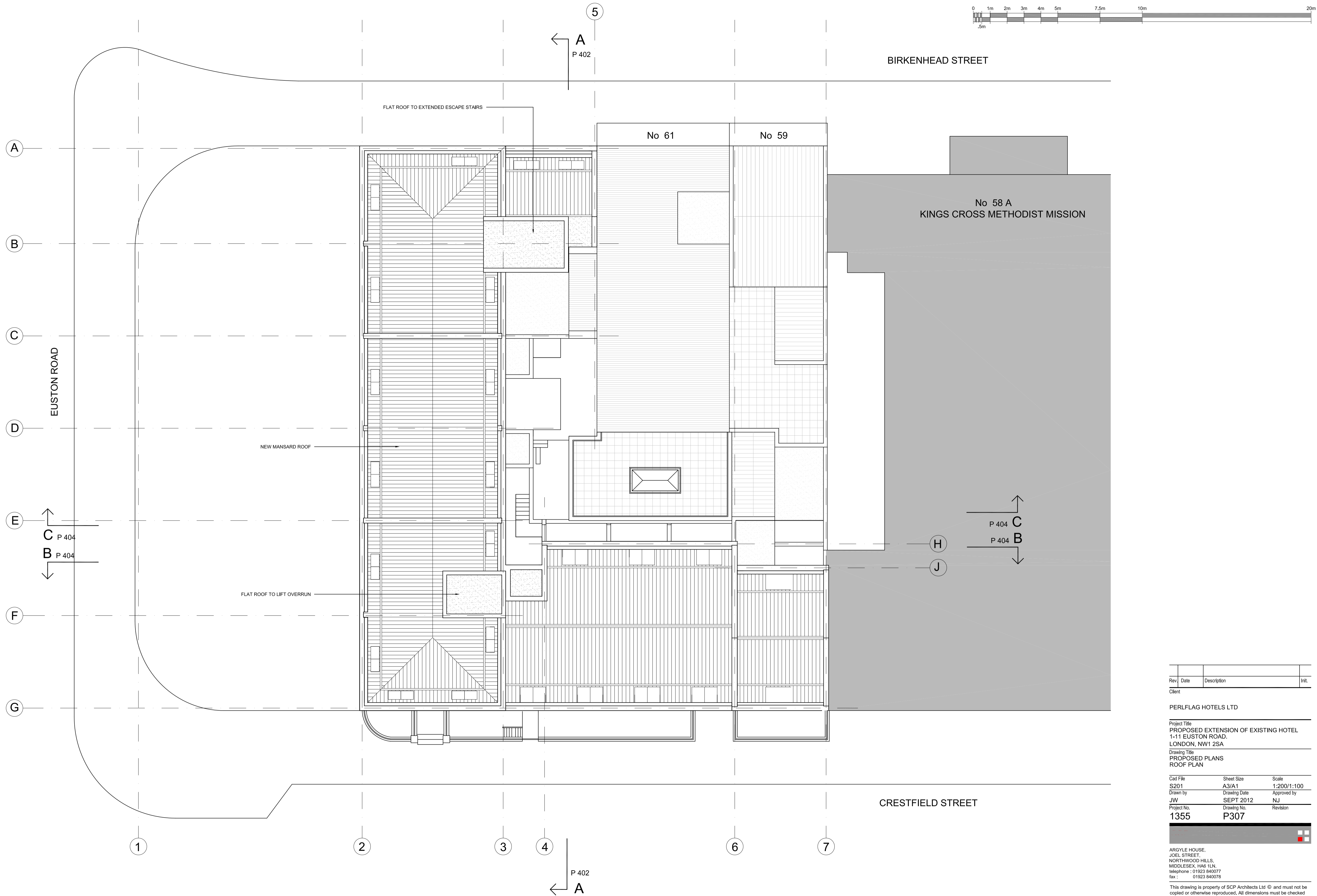
PROPOSED ROOF PLAN
