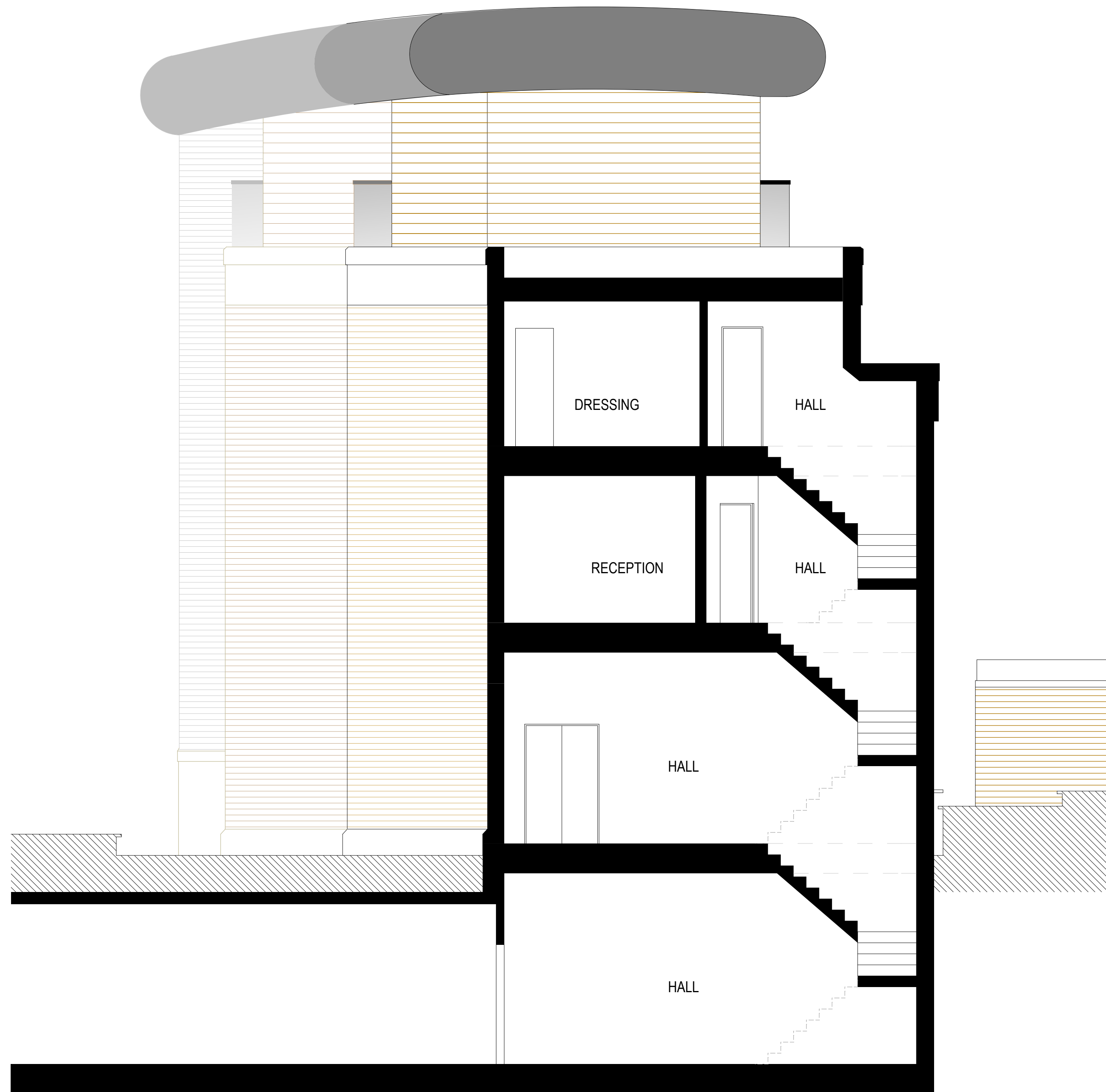
EXISTING SECTION A-A
