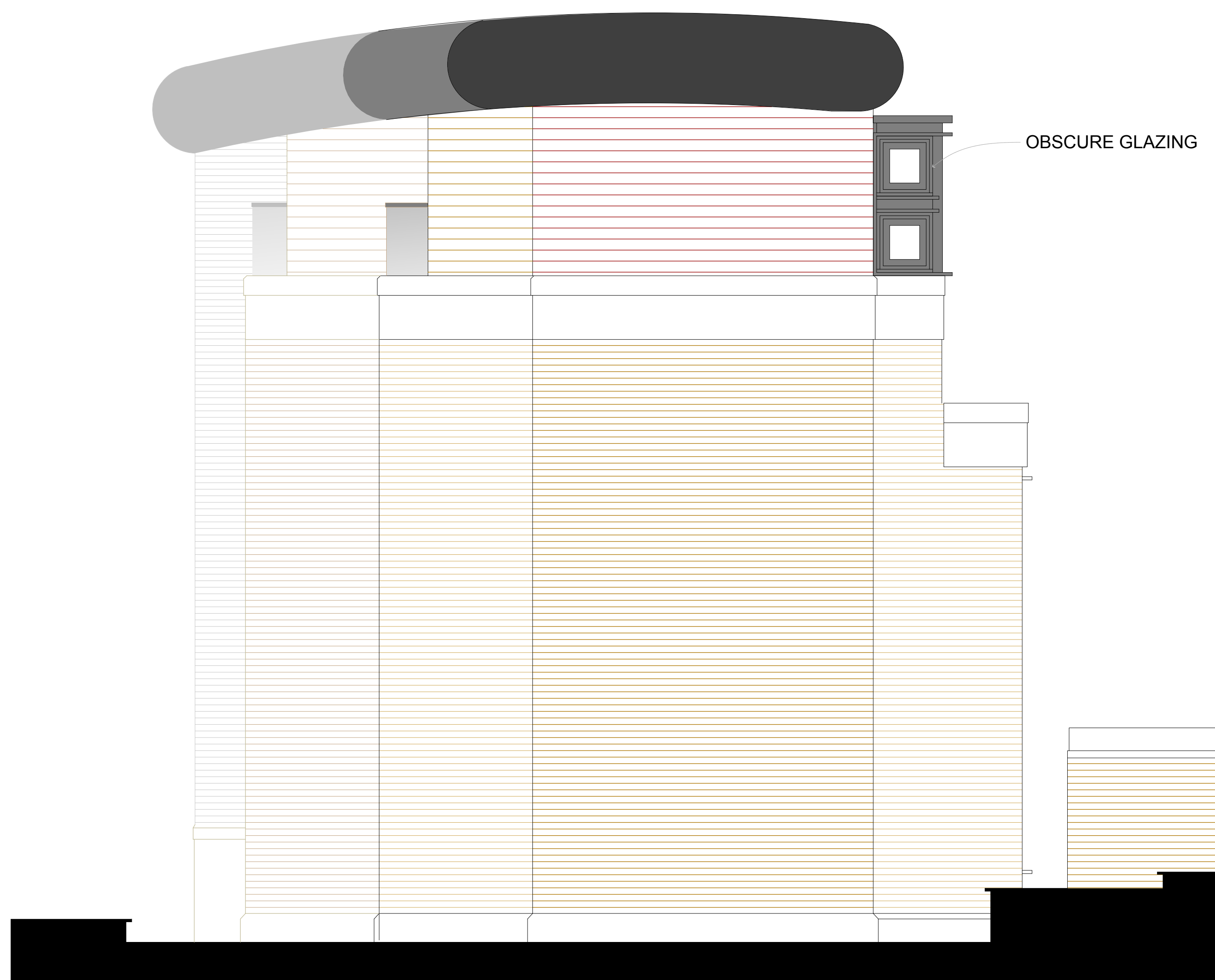
PROPOSED SIDE ELEVATION
