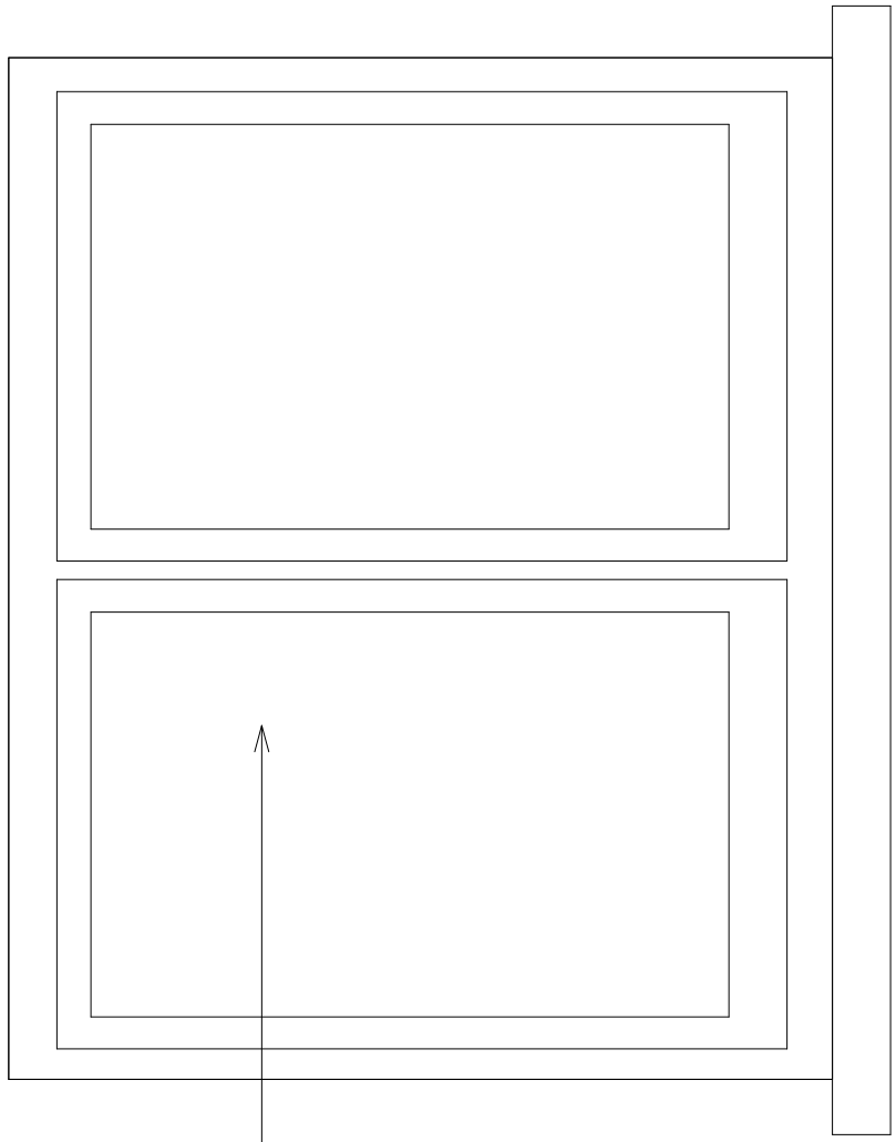
EXISTING THIRD FLOOR FRONT WINDOW (2NO.) SCALE 1:20
