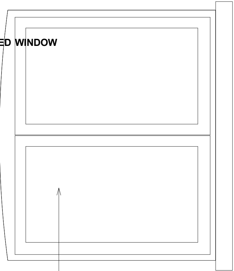
EXISTING THIRD FLOOR REAR WINDOW SCALE 1:20
