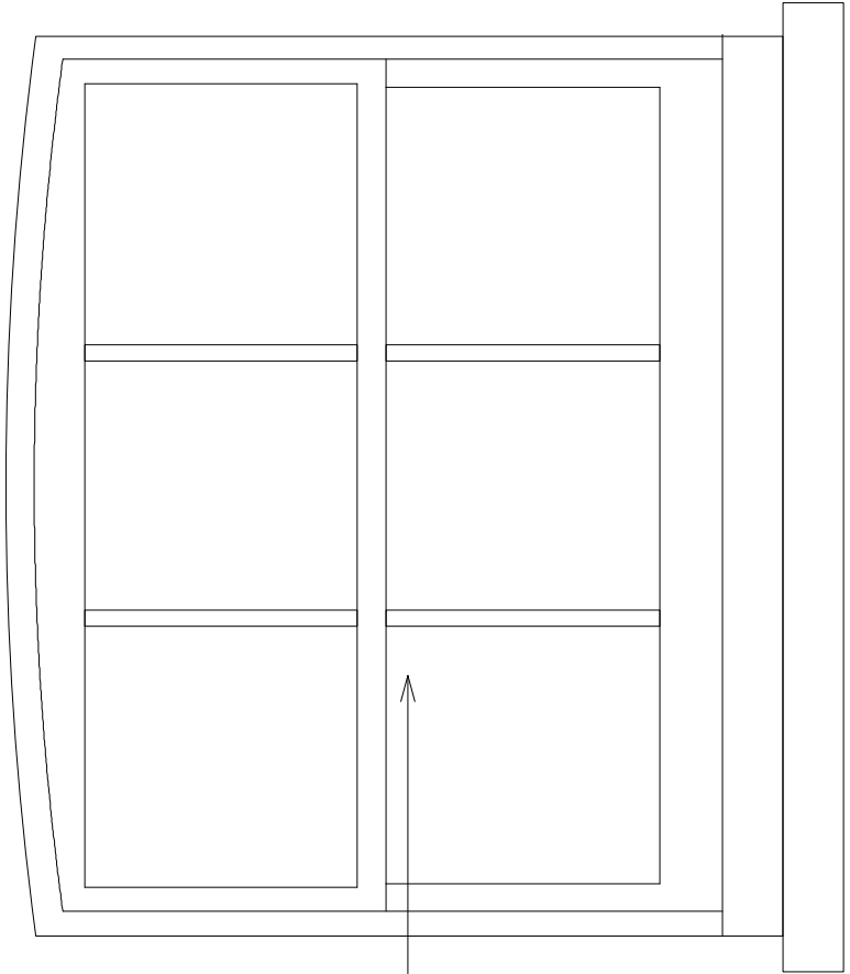
PROPOSED THIRD FLOOR REAR WINDOW SCALE 1:20
