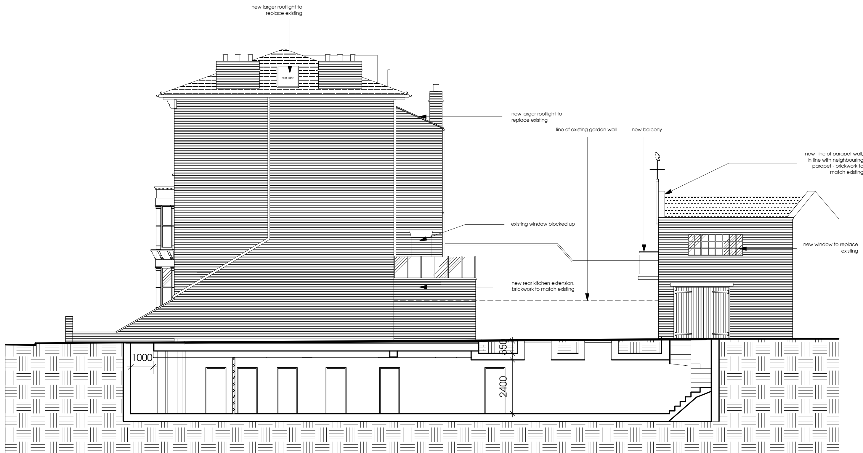
PROPOSED SIDE ELEVATION (SOUTH)
