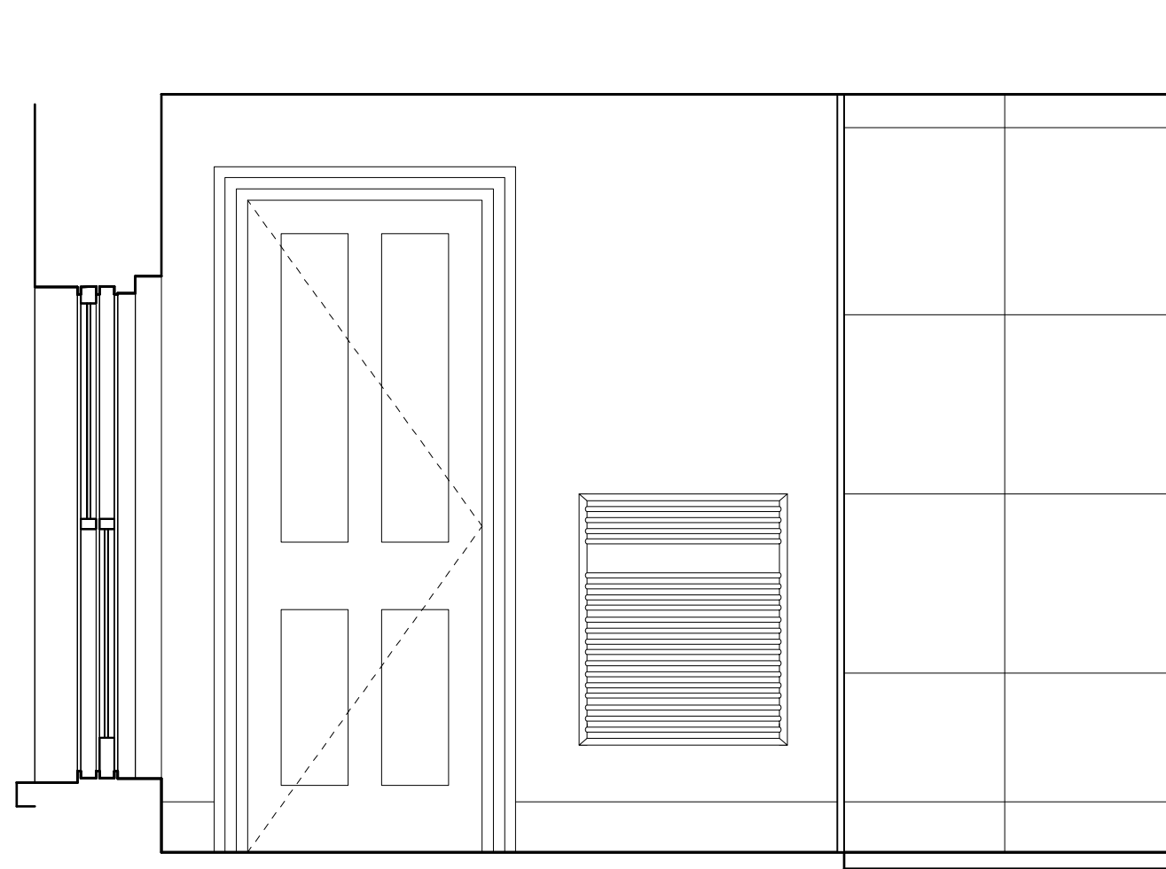
5 En Suite Elevation - Proposed Scale: 1:20
