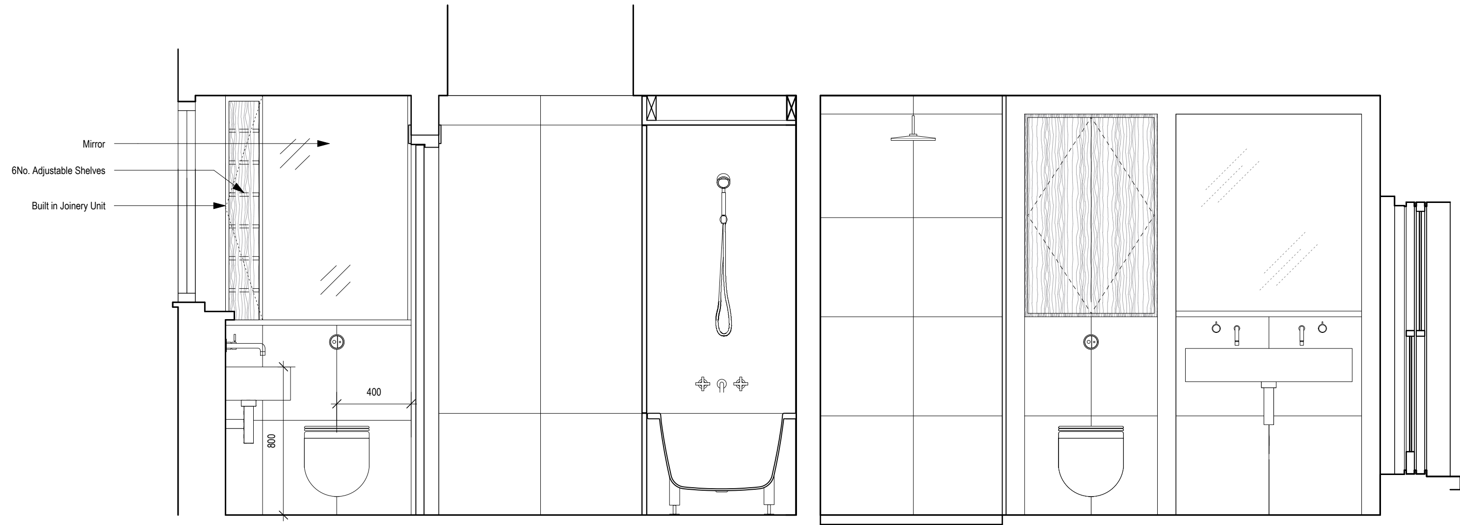
1 Family Bathroom Elevation - Proposed Scale: 1:20
