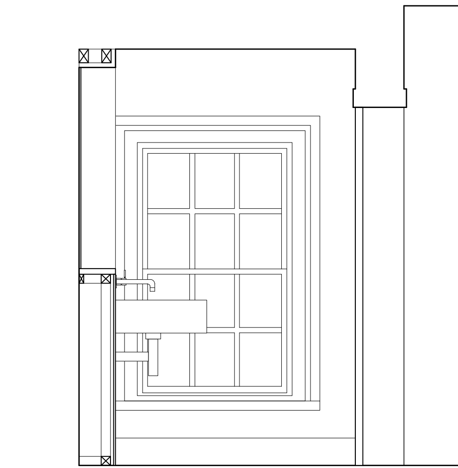
3 En Suite Elevation - Proposed Scale: 1:20
