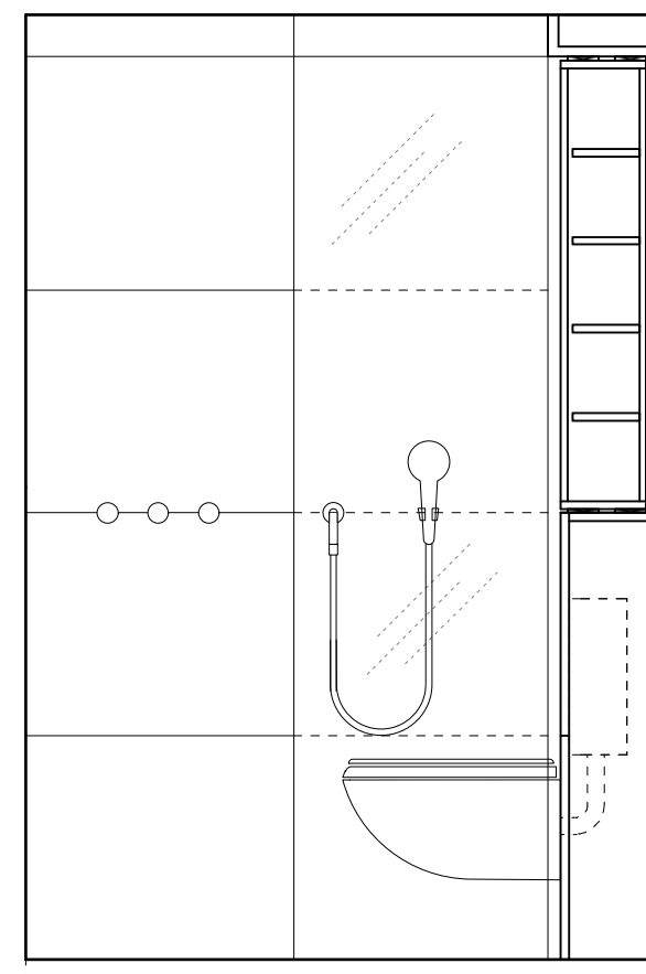
7 En Suite Elevation - Proposed Scale: 1:20
