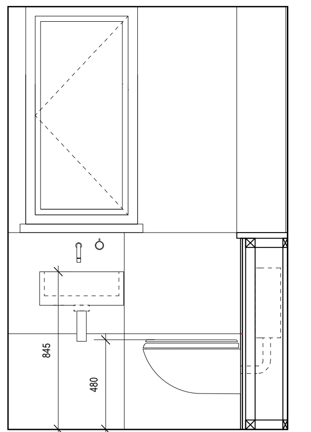
9 Family Bathroom Elevation - Proposed Scale: 1:20
