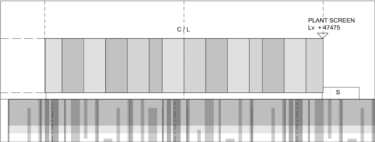
South Elevation of Plant Screen
