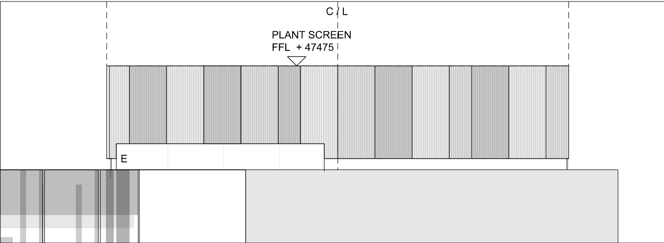
East Elevation of Plant Screen
