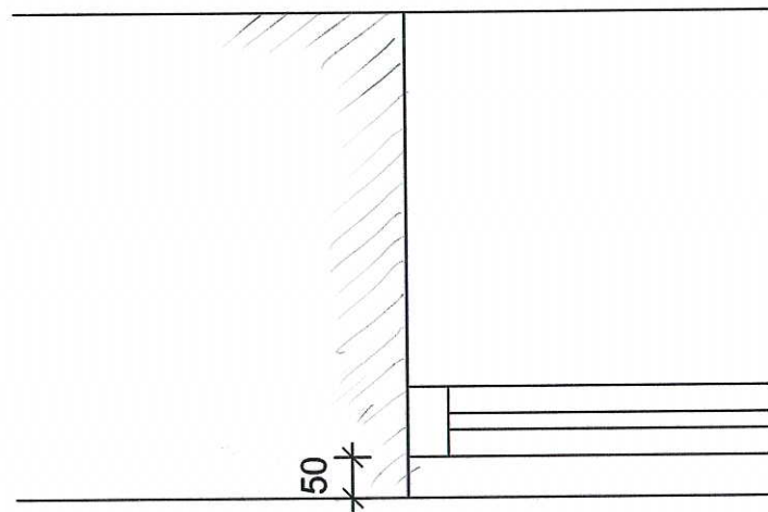
Window Reveal Scale 1:10
