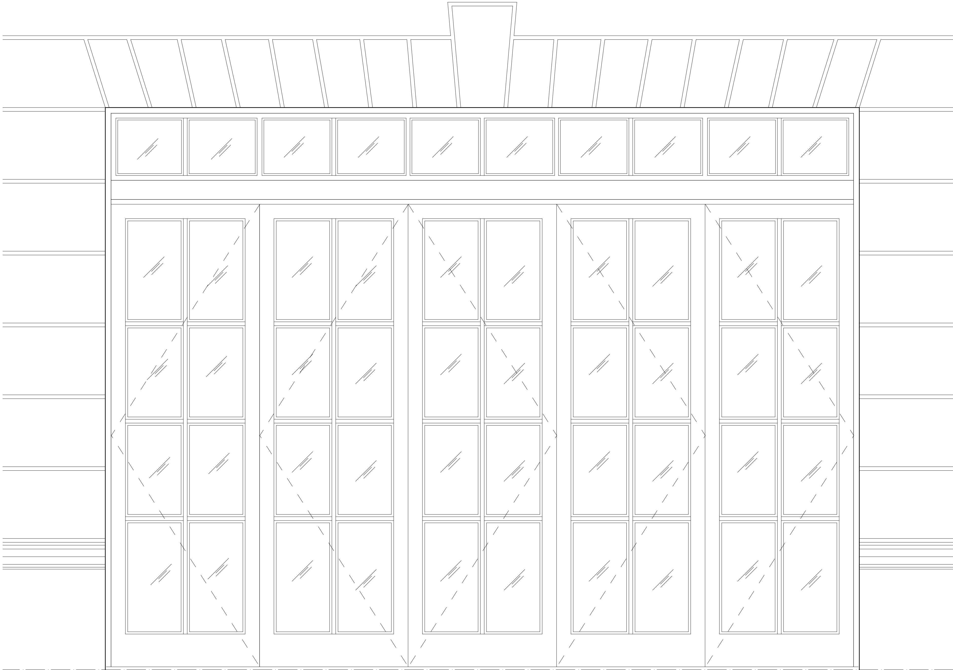
4 SCALE 1:10 @ A1 / 1:20 @ A3 TYPICAL GROUND FLOOR BIFOLD DOOR ELEVATION
