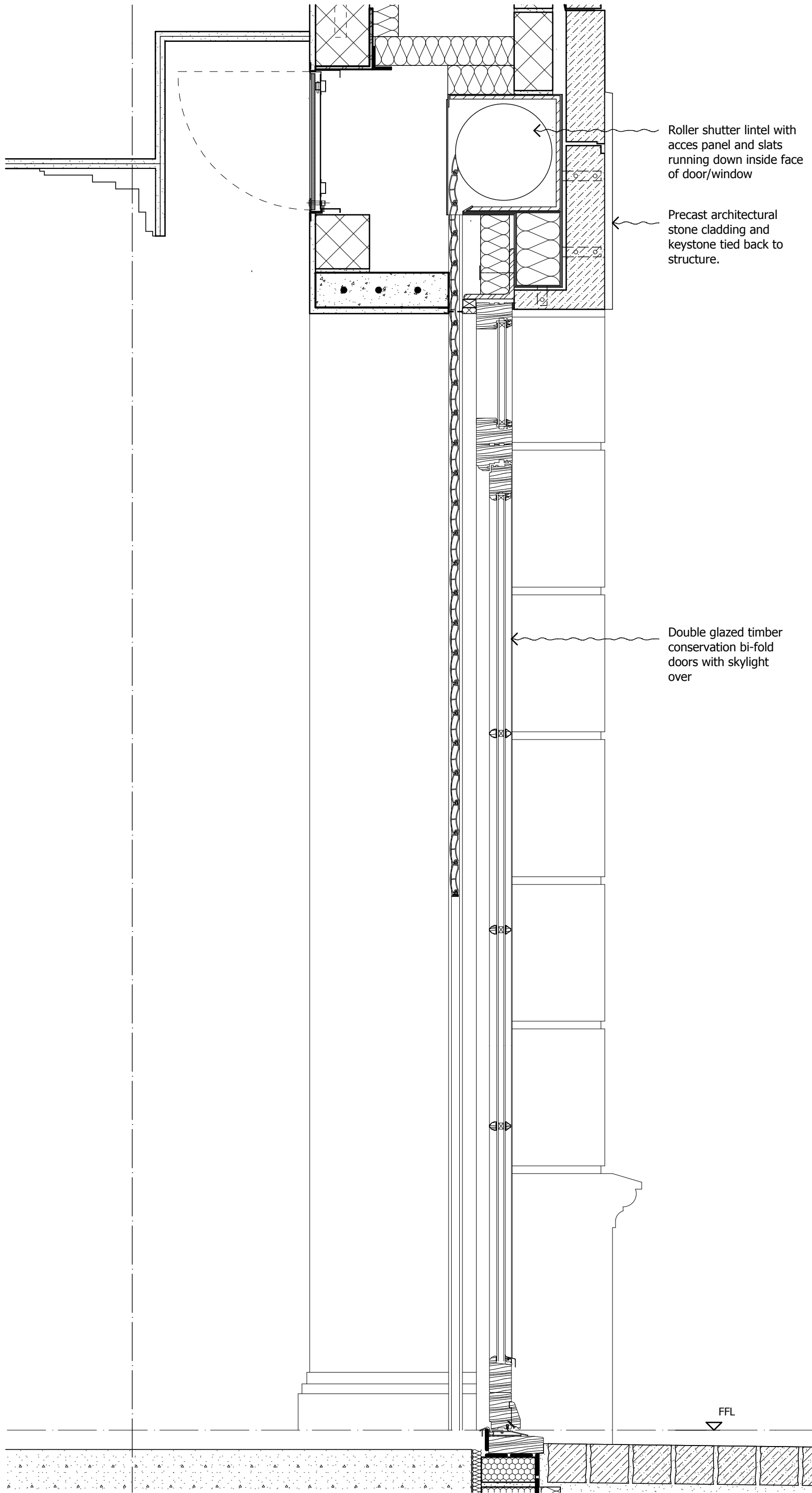
3 SCALE 1:10 @ A1 / 1:20 @ A3 TYPICAL GROUND FLOOR BIFOLD DOOR SECTION
