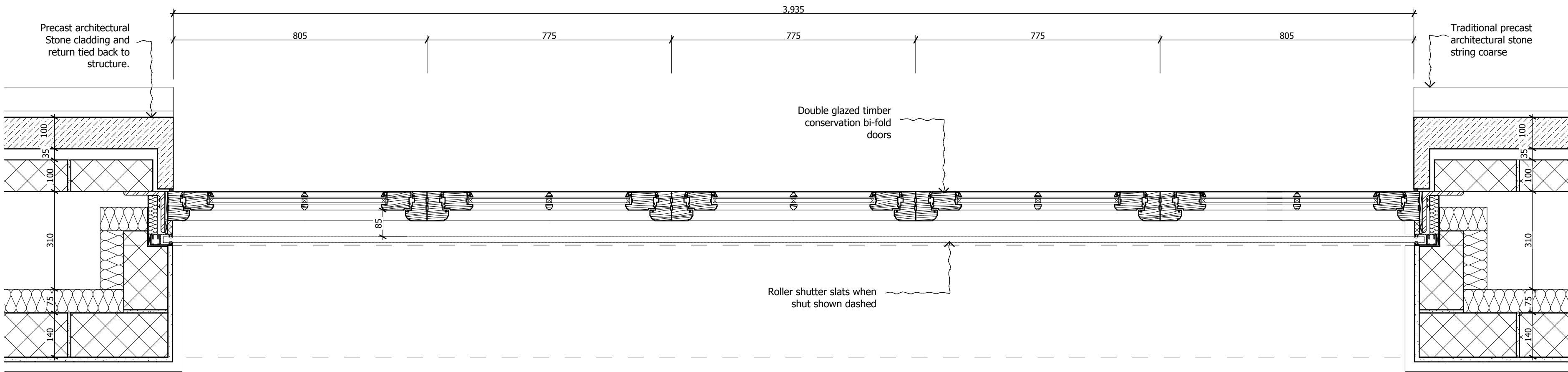
2 SCALE 1:10 @ A1 / 1:20 @ A3 TYPICAL GROUND FLOOR BIFOLD DOOR PLAN SECTION
