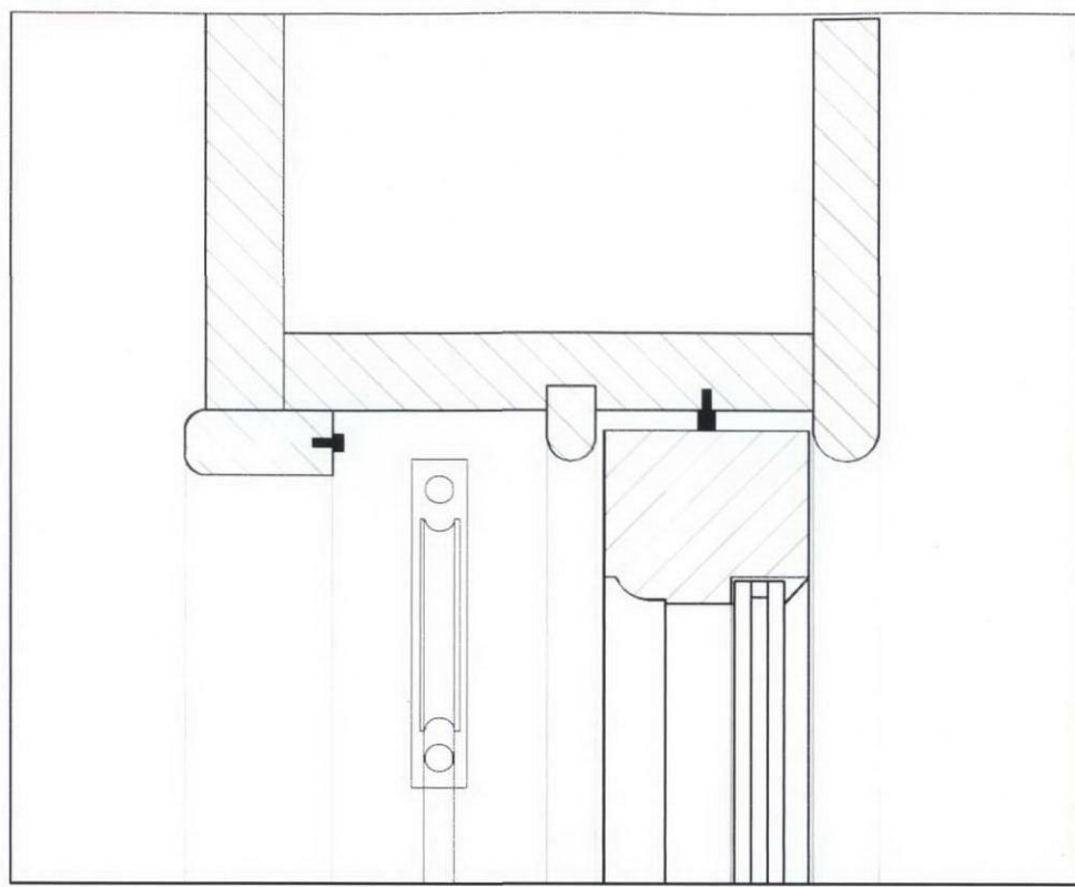
Head
