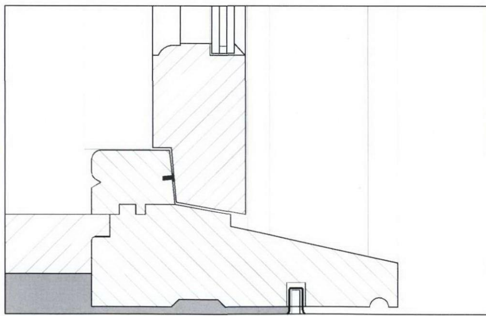
Sill
