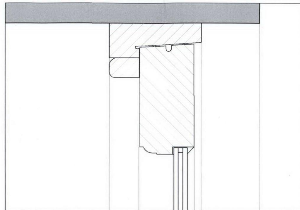
Head
