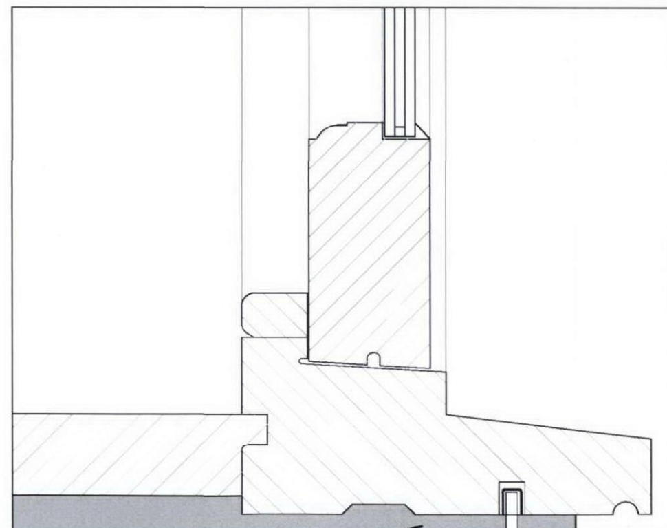
Sill
